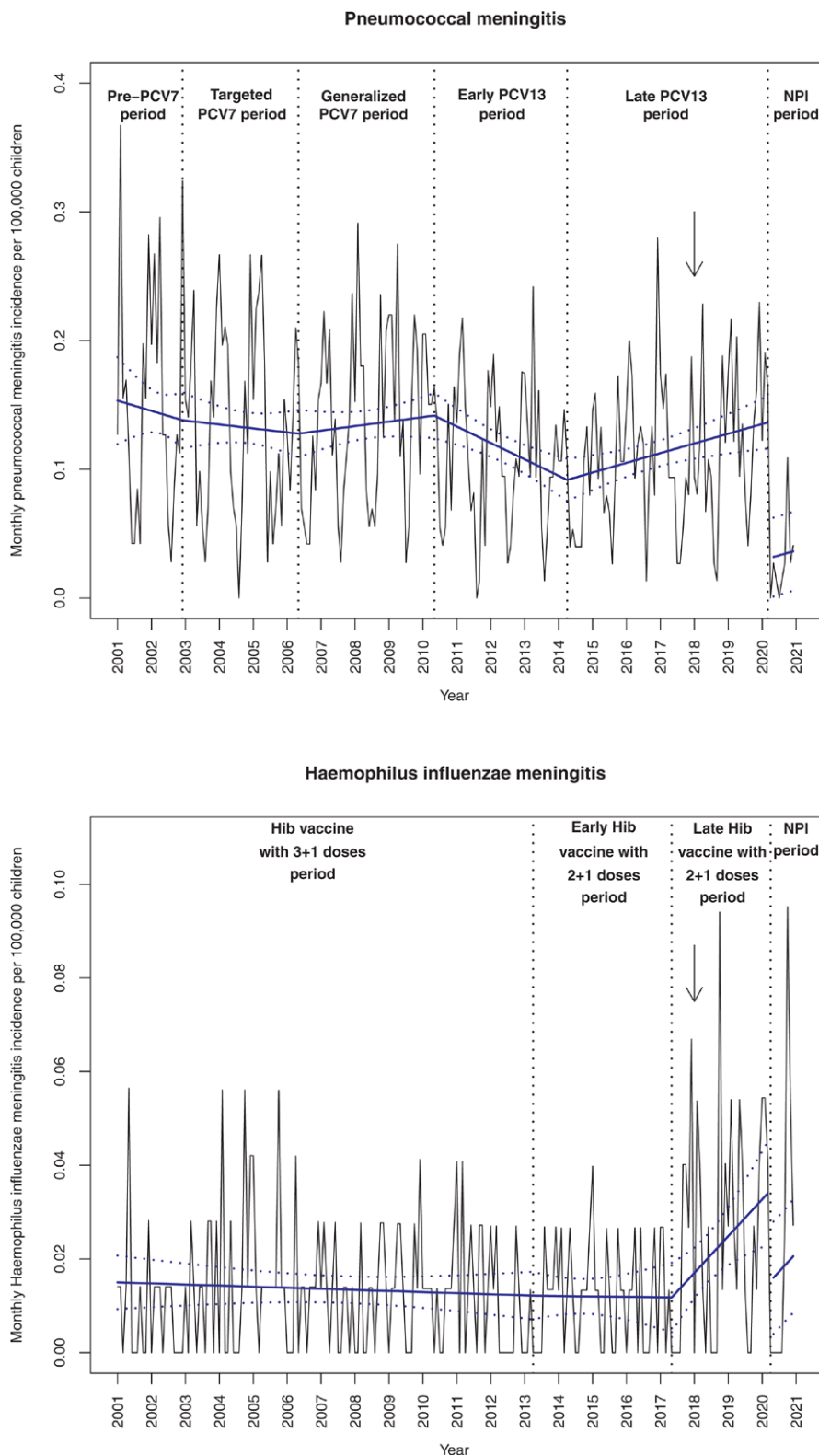
FIGURE 2. Monthly incidence per 100,000 children 15 years of age and younger for pneumococcal, and Haemophilus influenzae acute bacterial meningitis over time. Complete PCV vaccination at 24 months remained <80% until 2007. Complete Hib vaccination at 24 months was about 88% until 2013 and about 92% after. Since January 2018 (black arrows), 13-valent pneumococcal conjugate vaccine and H. influenzae serogroup b have become mandatory for children <2 years, leading to an increase in vaccine coverage. The “pre-PCV7 period” was from January 2001 to December 2002, the “targeted PCV7 period” from January 2003 to May 2006, the “PCV7 period” from June 2006 to May 2010, the “early PCV13” period from June 2010 to April 2014, and the “late PCV13” period from May 2014 to March 2020. The “Hib vaccine with 3 + 1 doses period” was from January 2001 to April 2013, the “early Hib vaccine with 2 + 1 doses period” from May 2013 to May 2017, and the “late Hib vaccine with 2 + 1 doses period” from June 2017 to March 2020. The “NPI period” was from April 2020 to December 2020. The black lines show the observed data. The blue slope lines were estimated with a segmented regression model. The blue dotted lines show the 95% confidence interval estimated with the segmented regression model. Hib indicates Haemophilus influenzae type b, NPI, non-pharmaceutical intervention; PCV, pneumococcal conjugate vaccine.
