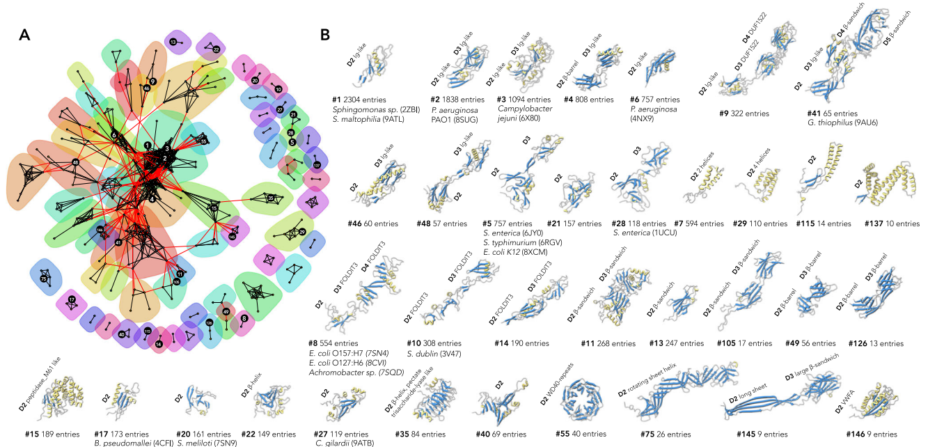
Fig. 5 | Populated flagellin outer domains in the bacterial domain. A The relationships among 682 structural clusters are depicted using the Fruchterman-Reingold algorithm, a force-directed layout algorithm from the R/igraph package. The communities, indicated with transparent color circles, were detected using the walktrap algorithm with a step size of 6. Additionally, some most populated clusters, as illustrated in (B) , are highlighted with black circles. B AlphaFold predictions
