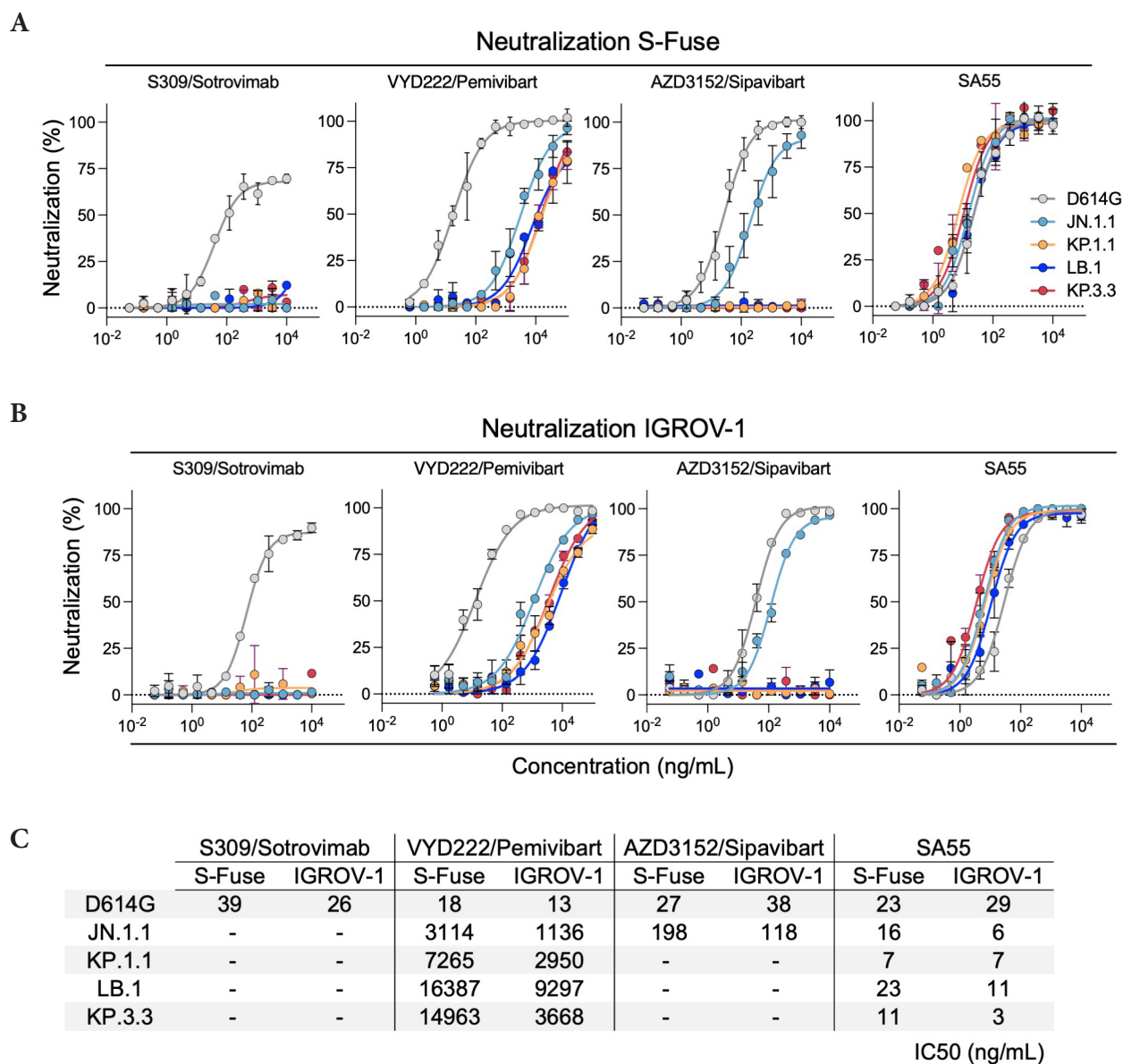
Figure 2. Neutralization of SARS-CoV-2 variants circulating in mid-2024 by mAbs. A. Neutralization curves of mAbs in S-Fuse cells. Dose-response analysis of neutralization of the indicated variants by S309/Sotrovimab, VYD222/Pemivibart, AZD3152/Sipavibart, and SA55. Data are presented as mean \pm standard deviation of 2-3 independent experiments. B. Neutralization curves of mAbs in IGROV-1 cells. Dose-response analysis of neutralization of the indicated variants by S309/Sotrovimab, VYD222/Pemivibart, AZD3152/Sipavibart, and SA55. Data are presented as mean \pm standard deviation of 2-3 independent experiments. C. EC50 values (in ng/mL) for each mAb against the indicated viral strains in the 2 cell lines. “-”: no antiviral activity.
