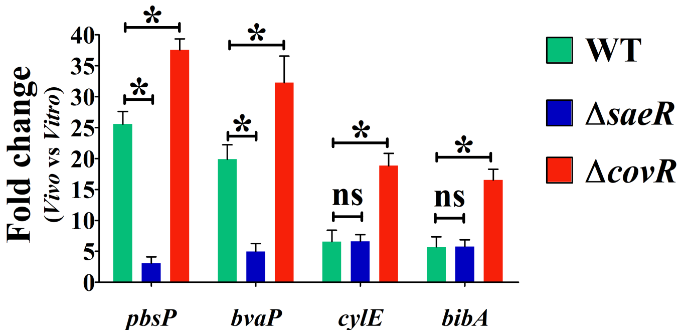
FIG 5 SaeRS is the main regulator of pbsP and bvaP expression in vivo . Transcription of virulence factors is quantified by RT-qPCR from bacteria recovered in PLF 1 h after intraperitoneal infection of mice and compared to in vitro growing bacteria. Transcription of positively SaeR-regulated genes ( pbsP , bvaP ) and negatively CovR-regulated genes ( cyle , bibA ) in NEM316 WT strain (green), \Delta saeR (blue), and \Delta covR (orange) mutants is normalized against gyrA , and expressed as fold change between in vitro and in vivo growth. Results are means \pm SDs from three independent experiments performed in triplicate. * P < 0.05; ns, non-significant, as determined by Mann-Whitney statistical analysis.
