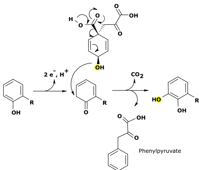
Fig. 5. Proposed molecular mechanism of prephenate-dependent hydroxylation: the reaction exemplifies the first hydroxylation step in the \text{O}_2 -independent biosynthesis of UQ 8 . R, octaprenyl chain.
