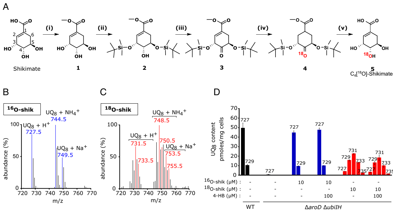
Fig. 4. Addition of \text{C}_4[^{18}\text{O}] -shikimate to the \Delta\text{aroD} strain leads to the biosynthesis of ^{18}\text{O}_3 -UQ in anaerobic conditions. (A) Synthetic route of ^{18}\text{O} -shikimate (3R,4S,5R)-3,4- [^{18}\text{O}] ,5-trihydroxy-4-cyclohex-1-ene-1-carboxylic acid. i) APTS, \text{CH}_3\text{OH} ; ii) TBDMSOTf, 2,6-lutidine, \text{CH}_2\text{Cl}_2 ; iii) Dess-Martin Periodinane, \text{CH}_2\text{Cl}_2 , rt; iv) \text{H}_2^{18}\text{O} , \text{CH}_3\text{C}[^{18}\text{O}]_2\text{H} , THF; v) a) \text{NaBH}_4 , THF/ \text{H}_2\text{O} ; b) APTS, THF/ \text{H}_2\text{O} . Mass spectra of UQ 8 from \Delta\text{aroD } \Delta\text{ubiIH} strain grown anaerobically in the presence of 10 μM unlabeled ^{16}\text{O} -shikimate (B) or \text{C}_4[^{18}\text{O}] -shikimate (C). The peaks corresponding to adducts of either unlabeled UQ 8 or UQ 8 labeled with two ^{18}\text{O} ( ^{18}\text{O}_2 -UQ 8 ) or three ^{18}\text{O} ( ^{18}\text{O}_3 -UQ 8 ) are represented in blue (B) and red (C), respectively. Mass spectra representative of three independent experiments. (D) Quantification of UQ 8 \text{H}^+ adducts ( m/z 727 to 735) in WT and \Delta\text{aroD } \Delta\text{ubiIH} cells grown with ^{16}\text{O} -shikimate or \text{C}_4[^{18}\text{O}] -shikimate. Mean \pm SD ( n = 3 ), see also SI Appendix, Fig S3 .
