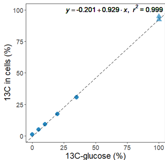
Fig. 1 Isotopic composition of E. coli cells, as determined by EA-IRMS, in function of the percentage of ^{13}\text{C}_6 -D-glucose employed in the D-glucose substrate. There are 4 replicates by condition. The different shapes, circles, and triangles represent two distinct experimental series. The dotted line and the equation shown in the plot are related to the linear regression
