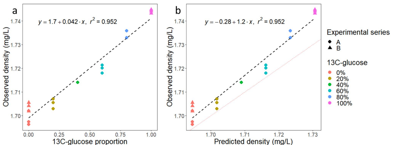
Fig. 2 Buoyant density of T4 bacteriophage DNA measured in CsCl gradient. a T4 DNA density as a function of the proportion of ^{13}\text{C}_6 -D-glucose employed in the D-glucose substrate for host growth. b T4 DNA density as a function of the theoretical density calculated according to the equation presented in the text [10]. The identity line is shown with red dots. The dashed line and equations shown on the plots are related to the linear regressions. The data originate from 2
