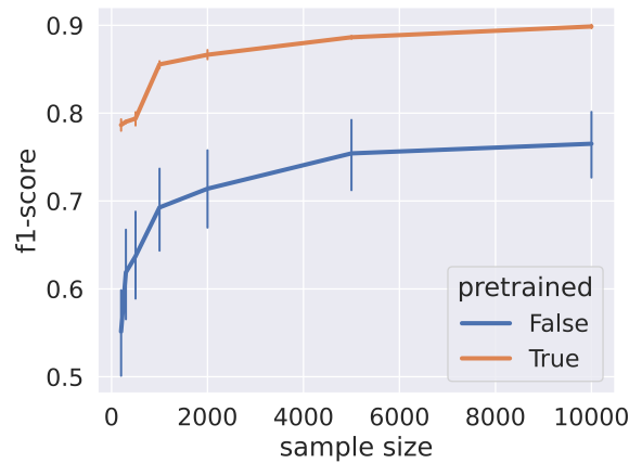
FIG. 3. f_1 -scores for different training dataset sizes (abscissa), with the MaggotUBA encoder pre-trained (orange) or not (blue). Train and test datasets were drawn from the new optogenetic screen. Pre-training was performed on [6, 10].
