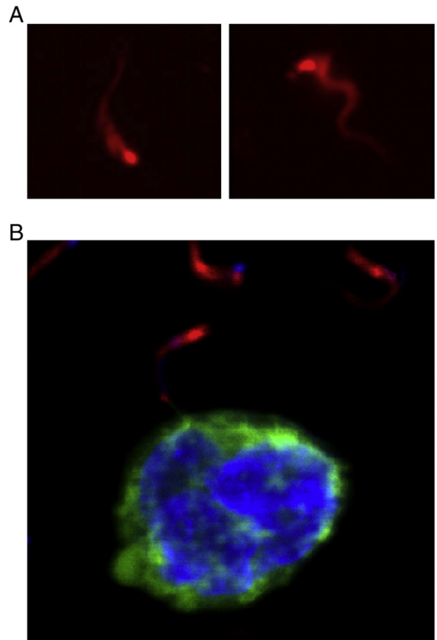
Fig. 7. Engineering TcTRES-Crim strain for multicolor applications. Epimastigote (left panel) and trypomastigote (right) forms of Y strain of T. cruzi (A); TcTRES-Crim parasites were pictured in the presence of human acute monocytic leukemia cell line (THP-1) stained with green fluorescence cell dye (pKH2) and DAPI, for contrast.
