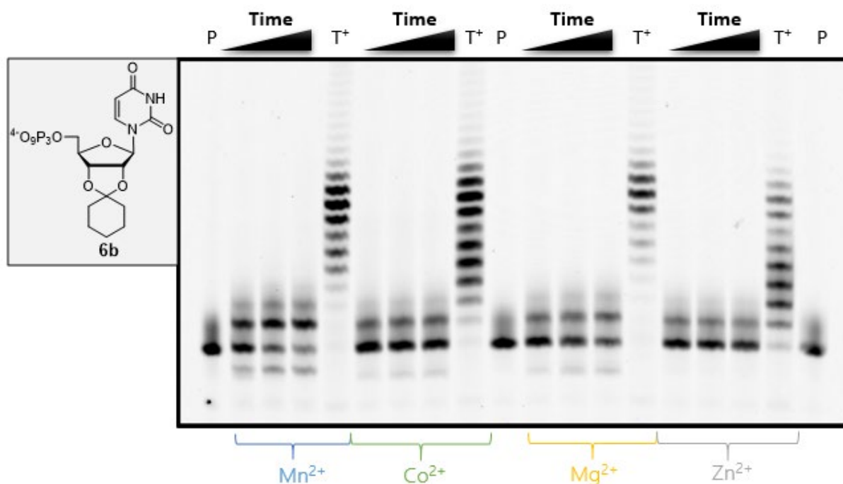
Figure 1. Gel (PAGE 20%) analysis of PEX reaction of 2',3'-O-cyclohexylidene-UTP 6b . All reactions were incubated with 1 mM of 6b , 20 pmol of RNA primer, 10 U of PUP, 1 mM of metal ( Mn^{2+} , Co^{2+} , Mg^{2+} , Zn^{2+} from left to right), 20 U RNase Murine Inhibitor varying reaction time (i.e. 1 h, 3 h, 5 h) at 37°C. Control reactions were carried out in the presence of unmodified UTP for 1h (T+) or primer only (P).
