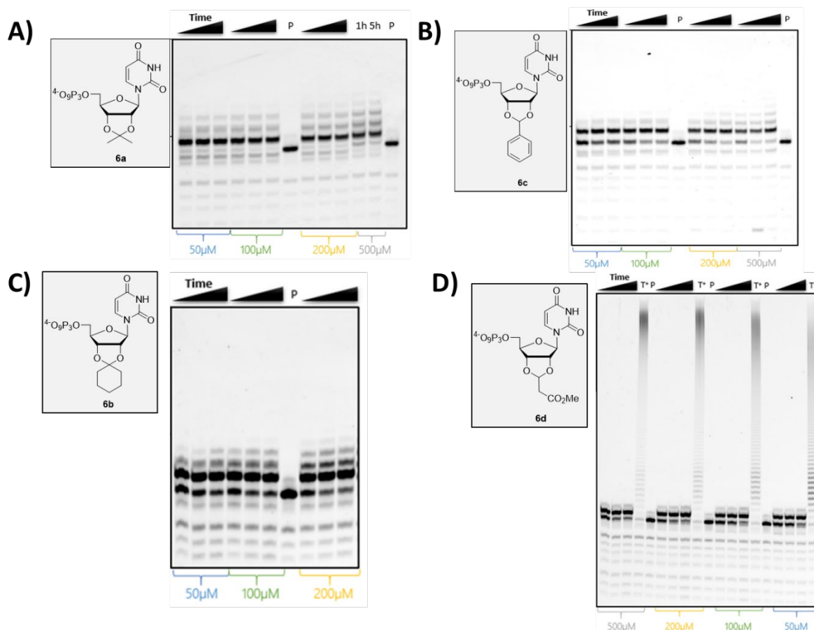
Figure 3. Gel (PAGE 20%) analysis of PEX reaction of N*TP-UTP 6a , 6b , 6c and 6d with concentration from 50 to 500 \mu\text{M} . All reactions were incubated with 10 pmol of RNA primer, 10 U PUP, 1 mM of \text{Mn}^{2+} , 20 U RNase Murine Inhibitor varying reaction time A), B) and C) (i.e. 1 h, 3 h, 5 h) or D) (i.e. 30 min 1 h, 3 h) at 37°C. Primer only (P).
