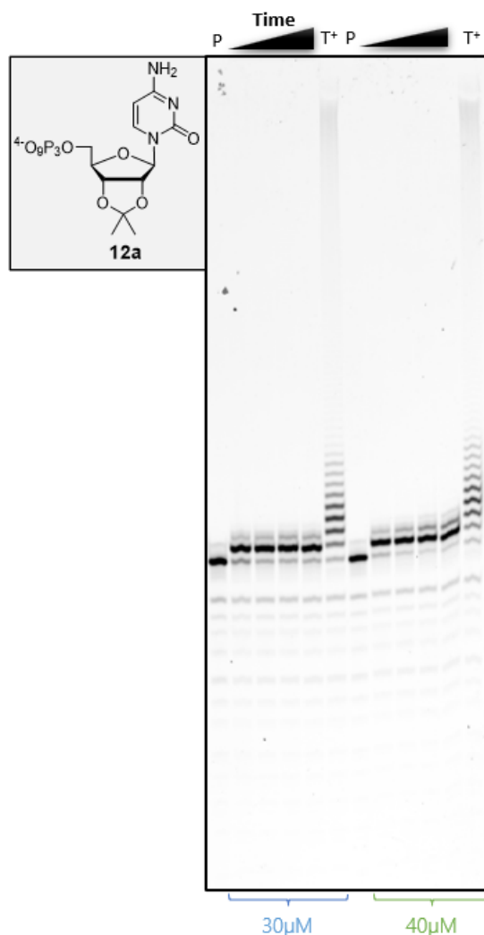
Figure 5. Gel (PAGE 20%) analysis of PEX reaction of 2',3'-O-isopropylidene CTP 12a . A) Concentration of 12a at 30 or 40 \mu\text{M} at various reaction time (i.e. 1 min 45, 5, 15, 30 min). All reactions were incubated with 10 pmol of RNA primer, 10 U PUP, 1 mM of \text{Mn}^{2+} , 20 U RNase Murine Inhibitor at 23°C. Primer only (P).
