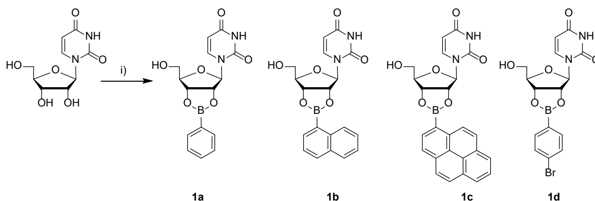
Scheme 2. Synthesis of uridine nucleosides with boronic ester protecting groups. Reagents and conditions: i) a) RB(OH) 2 , pyridine, reflux, 4-5 h, MgSO 4 ; b) Precipitation in CH 3 CN; 39% ( 1a ), 43% ( 1b ), 87% ( 1c ), 74% ( 1d ).
