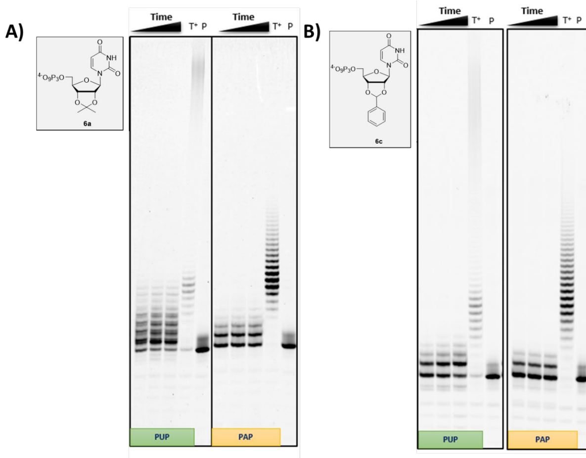
Figure 2. Gel (PAGE 20%) analysis of PEX reaction of 2',3'-O-isopropylidene-UTP 6a and 2',3'-O-benzylidene-UTP 6c . All reactions were incubated with 1 mM of N*TP, 20 pmol of RNA primer, 10 U of PUP or PAP, 1 mM of Mn 2+ , 20 U RNase Murine Inhibitor varying reaction time (i.e. 1 h, 3 h, 5 h) at 37°C. Control reactions were carried out in the presence of unmodified UTP for 1 h (T+) or primer only (P).
