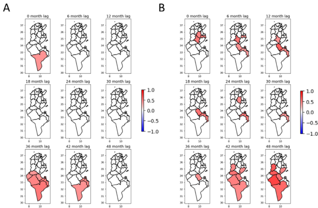
268 Fig. 5: (A) Significant full series correlations ( p -value < 0.05) of NAO vs. Rainfall (smoothed with 12-mo moving 269 windows) in Tunisia at the province level from 2007 to 2021. (B) Significant correlations ( p -value < 0.05) NAO vs ZCL 270 (smoothed with a 12-mo moving average) in Tunisia at the provincial level for the period 2007-2021 271 272 273
