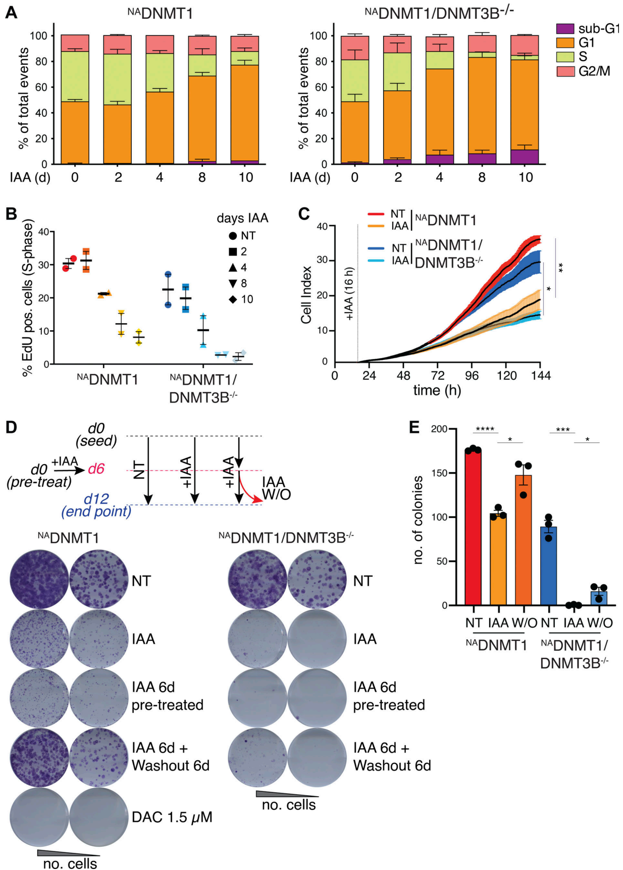
Figure 3. DNMTs degradation impairs cell proliferation. (A) Cell cycle profiling by EdU/DAPI incorporation upon induced DNMT1 degradation at the indicated days from IAA treatment in DLD-1 NADNMT1 (left) and NADNMT1/DNMT3B -/- cells. N = 2, Error bars represent SEM. (B) Quantification of S phase (% of total events)
