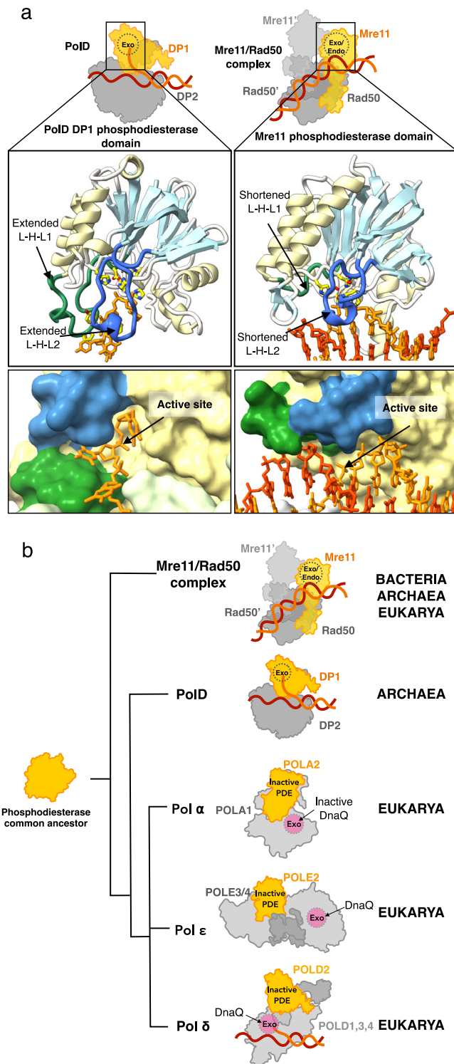
Fig. 6 | Evolutionary implications of the PDE-fold across proteins and Domains of life. a Top: Schematic representations showing the nuclease active sites in PolD (left) and Mre11/Rad50 (right). Middle: Cartoon representation of the PDE domain of PolD (left) and Mre11/Rad50 (right). The \alpha -helices are represented in yellow and the \beta -sheets in light blue to illustrate the shared structural topology of their PDE domains. The loop-helix-loop motifs 1 and 2 (L-H-L 1 and 2) are highlighted in green and dark blue, respectively. Bottom: Surface representation of the PolD exo channel (left) and the corresponding region in Mre11/Rad50 (right). The ssDNA substrate is represented by the black arrow and the L-H-L 1 and 2 motifs are highlighted in green and dark blue, respectively. b Putative evolutionary scenario of the PDE domain in Mre11 and DNA polymerases from a common ancestor. An active PDE motif has been retained in archaeal PolD, as well as in Mre11, a ubiquitous exo/endonuclease found in all three domains of life. Through evolution, the PDE motif became inactivated in eukaryotic repDNAPs as they acquired the Dna-Q-like exonuclease domain.
