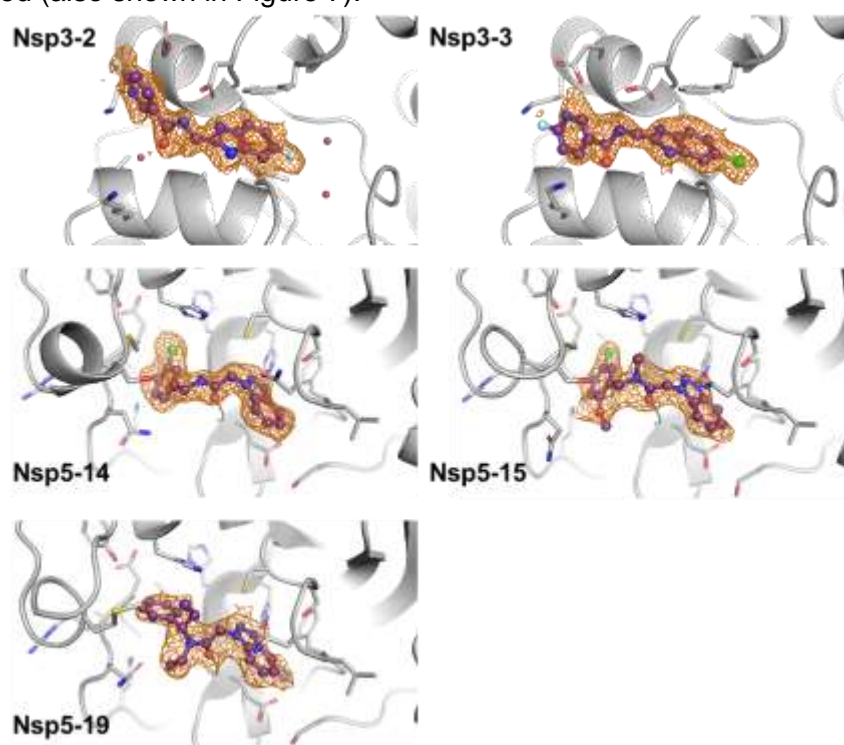
Figure 7. Crystal structures with examples of the Nsp5 benzotriazolyl acetamide family and Nsp3 (macrodomain) binders. The compounds are shown with purple sticks and balls and the PanDDA event map is shown as an orange mesh. PDB files can be downloaded from https://github.com/hermanslab/COVID-19 .
