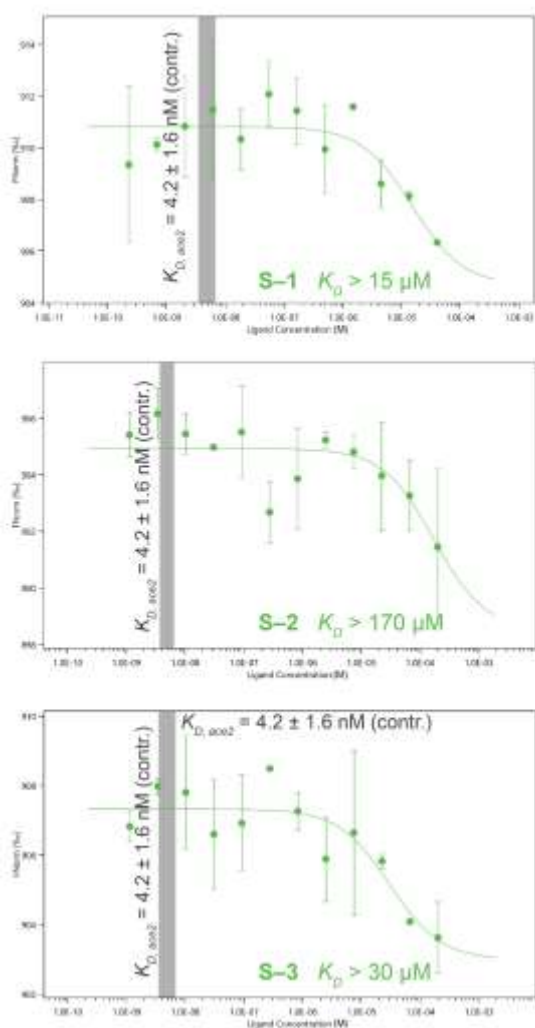
Figure 6. Binding curves of S compounds using Microscale thermophoresis performed in triplicate. Error bars show standard deviations. The gray region shows the K_D for positive control Ace2. See Supporting Information Section 4.2 for details on assay conditions.
