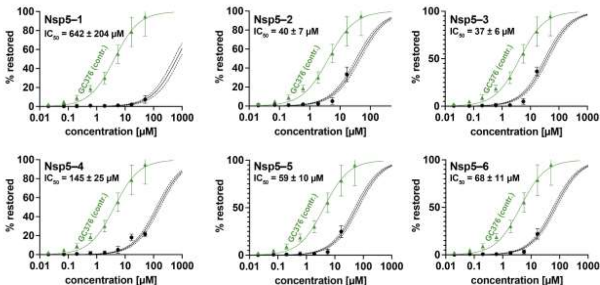
Figure 5. Dose-response curves of compounds in cell-based Nsp5 protease assay. IC_{50} values are also in Table 3 below. Solid line: curve fit result. Dashed lines: 95% confidence interval. Data are expressed as the mean \pm standard deviation of 3 independent experiments each performed in triplicate. Green triangles show positive controls for inhibitor GC376 (see Supporting Information section 4.3.2). Cytotoxicity was detected above 20 \mu\text{M} , so higher concentrations were excluded.
