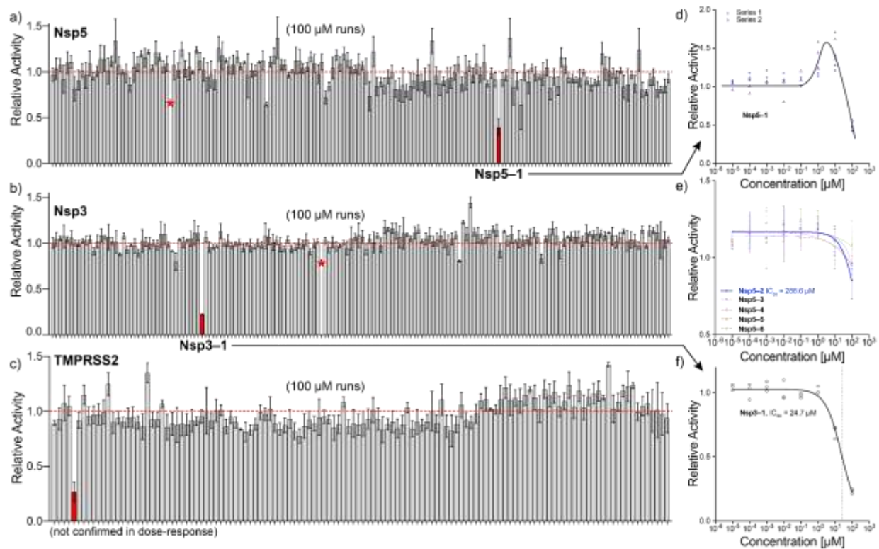
Figure 4. Overview of protease cleavage assays. a–c) relative activity over triplicate experiments at a fixed compound concentration of 100 \mu M for Nsp5, Nsp3 and TMPRSS2, respectively. Red bars show compounds that reduce cleavage (relative) activity by more than 50%. Asterisks show highly fluorescent compounds that could not be analyzed. Not all compound labels are listed for clarity. d–f) dose-response curves at different compound concentrations. Solid lines in panel e–f show fits, panel d to guide the eye.
