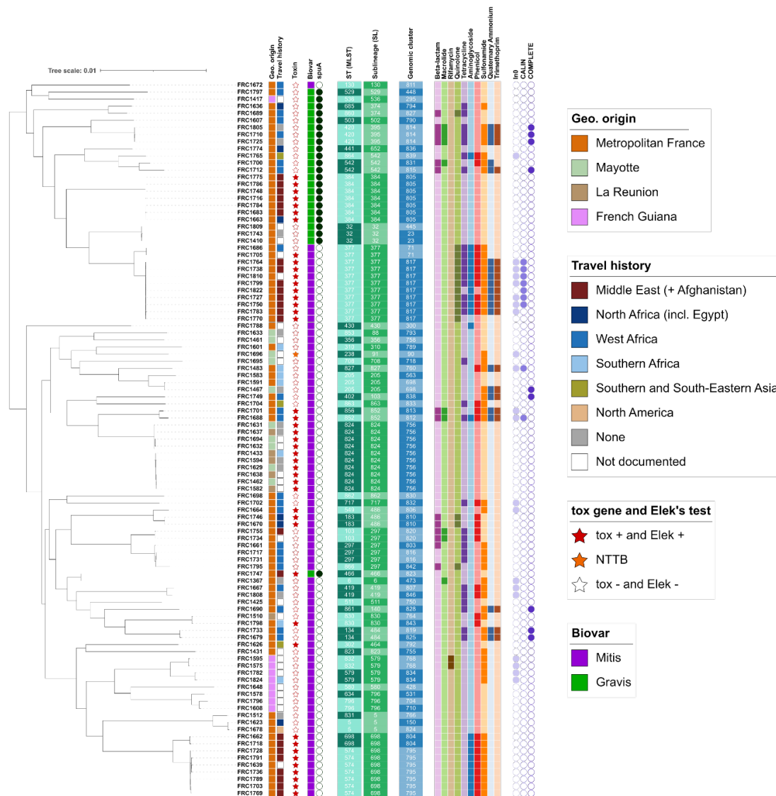
Figure 1 - Phylogenetic tree of Corynebacterium diphtheriae from France, 2022. The tree was obtained by maximum likelihood based on a multiple sequence alignment of the core genome. The scale bar represents the number of nucleotide substitutions per site. The first column that follows the isolates identifiers indicates the geographic origin (place of isolation; see key). Travel history provides the most distant geographic region of reported travel (see key); note that Afghanistan was included in Near and Middle East; and Egypt was included in North Africa. The stars represent the presence (red star), presence but disruption (NTTB, orange) or absence (white star) of the diphtheria toxin tox gene. Biovars are represented in colored squares, and spuA gene presence by a dark green circle. MLST STs, sublineage (SL) and genomic clusters are provided with an alternation of colored strips. Identifiers of the main STs are indicated (note the strong concordance between ST and cgMLST sublineages). The 10 next colored columns correspond to the presence of at least one gene or mutation (for quinolone and rifamycin classes) involved in resistance to the indicated class of antimicrobial agents. Last, the presence of integron-related structures (Cury et al., 2016) is indicated: In0 (integron integrase and no attC sites), CALIN (clusters of attC sites lacking integron-integrases) and complete integrons (integrase and at least one attC site). The simultaneous presence of In0 and CALIN may denote their presence in different contigs even though the integron might be complete.
