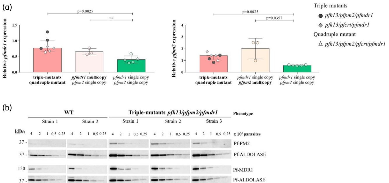
Figure 2. (a) Pfmdr1 and pfpfm2 expression in triple- and quadruple-mutant P. falciparum isolates. Pfmdr1 and pfpfm2 normalized expression levels were quantified in seven triple-mutant isolates (left histogram bar red bar and black dots, light grey diamonds and white triangle according to genotypes), five WT strains (right histogram bar green bar) and three Pfmdr1 single copy and three Pfpfm2 single copy isolates (middle histogram bar pink or orange bar). Each symbol corresponds to the mean value in one isolate (three replicates). Each bar corresponds to the median expression in quadruple, triple or double mutants and WT isolates (compared with the Mann–Whitney U -test). (b) Western blot analysis of Pf-PM2 and Pf-MDR1 expression in three Pfmdr1 triple mutants and two WT isolates. Pf-PM2 and Pf-MDR1 expression levels were assessed in synchronized P. falciparum trophozoites (24–30 h post-invasion). Pf-aldolase was used as loading control. This figure appears in colour in the online version of JAC and in black and white in the print version of JAC.
