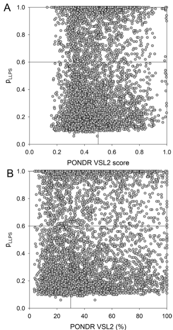
Fig. 11 Intrinsic disorder and phase separation propensity of 4792 human proteins interacting with all HIV-1 proteins. A p_{LLPS} vs. Pondered ® VSL2 disorder score dependence. In these analyses, proteins with p_{LLPS} \geq 0.6 are expected to serve as LLPS drivers, whereas proteins with the disorder scores \geq 0.5 are predicted as mostly disordered. Among the 4792 human proteins interacting with all HIV-1 proteins, 1738 proteins (36.27%) are expected to be mostly disordered, and 1669 (34.83%) are expected to serve as LLPS drivers. Among the LLPS drivers, 655 proteins (39.24%) are mostly disordered, indicating that 13.67% of HIV-1-interactors are mostly disordered proteins driving LLPS. B Dependence of the p_{LLPS} on the percent of disordered residues predicted by Pondered ® VSL2. Proteins with p_{LLPS} \geq 0.6 are expected to serve as LLPS drivers, whereas proteins with the PPIDR \geq 30\% are predicted as highly disordered. Based on the outputs of these analyses, 2820 human proteins from HIV-1 interactome (58.84%) are expected to be highly disordered. Among 1669 of LLPS drivers, 1038 proteins (62.19%) are expected to be highly disordered, indicating that 21.66% of HIV-1 interactors are highly disordered LLPS drivers
