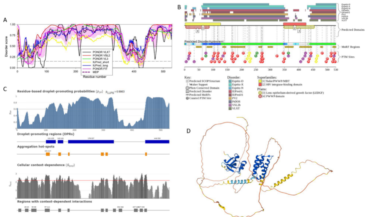
Fig. 6 Functional disorder analysis of human LEDGF/p75 protein (UniProt ID: O75475). A Per-residue disorder profile generated by RIDAO [138]. B Functional disorder profile generated by the D^2P^2 platform [139]. Here, phosphorylation, ubiquitylation, sumoylation, and acetylation sites are shown by red, violet, green and yellow circles with characters P, U, S, and A, respectively. An interactive profile generated for this protein by D^2P^2 is available at https://d2p2.pro/view/sequence/up/O75475 . C Evaluation of LLPS predisposition and existence of regions with context-dependent disorder [145]. D Model of the LEDGF/p75 structure generated by AlphaFold [147]
