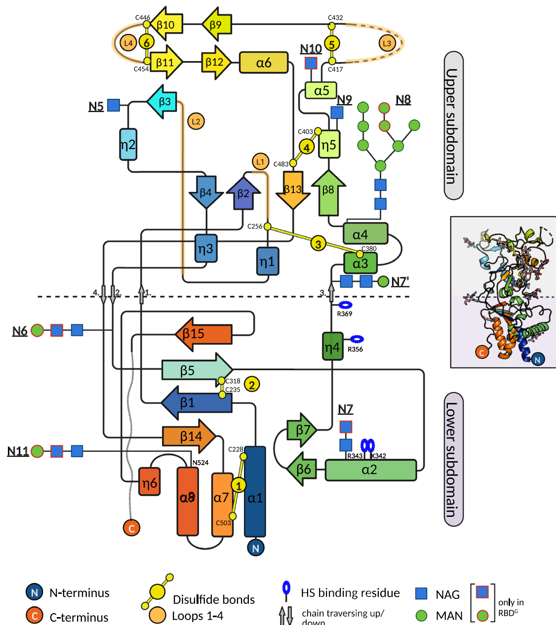
Fig. 2 | SFV RBD secondary structure topology diagram. The horizontal dashed-line designates the boundary between the lower and upper subdomains. The NAG and MAN units built only into the RBD G (and not RBD D ) structure are indicated with red frames. The figure was created with BioRender.com.
