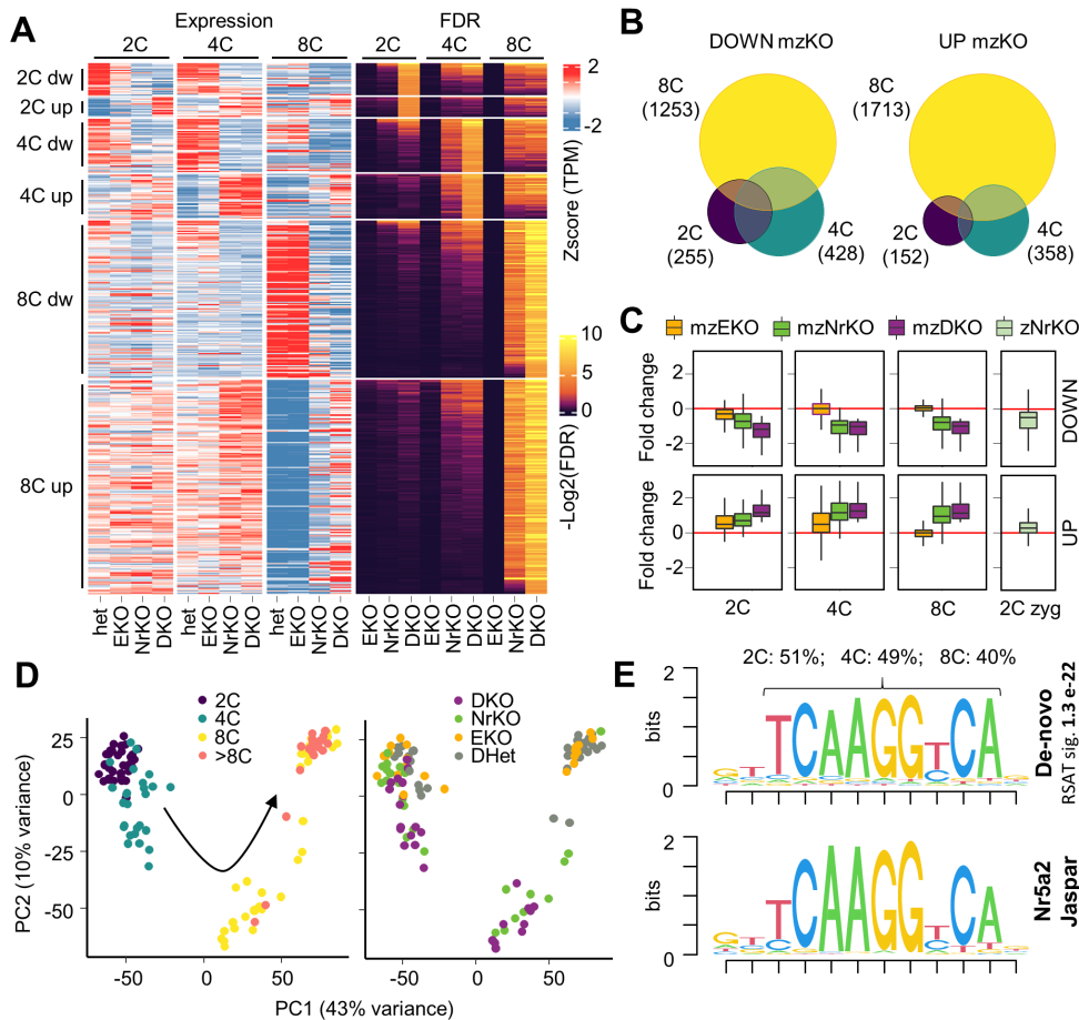
Fig. 3. Transcription is progressively deregulated in Nr5a2 KO embryos, from the 2C to the 8C stage. (A) Heatmap showing relative expression (Z-scores) of genes significantly affected - absolute FDR change > 1.5; False discovery rate (FDR) < 0.1; cutoff 10 transcripts per million (TPM) - after the loss of maternal and zygotic expression of Esrrb , Nr5a2 or both genes at the 2, 4 or 8-cell stage. (B) Number and overlap between the genes differentially expressed (as in A) in response to the loss of Esrrb , Nr5a2 or both genes at different stages of development. (C) Fold change in expression of genes significantly affected (as in A) in response to the maternal and zygotic KO of Nr5a2 and/or Esrrb . The fold change of the same set of genes in response to the zygotic knockout of Nr5a2 at the 2C-stage is shown alongside (2C zyg). (D) Principal component analysis of the transcriptome from individual embryos color coded to highlight differences in genotypes (right) or developmental stage (left). The black arrow intends to highlight an ideal progression along a pseudo-time of development. (E) ESRRB/NR5A2 binding sequence identified by de novo TF binding motif discovery over accessible regions surrounding the NR5A2-responsive genes in 2, 4 and 8C embryos, and NR5A2 binding consensus retrieved from the Jaspar database. The percentage of responsive genes (as in A) associated with an accessible region containing the NR5A2/ESRRB motif is reported at the top.
