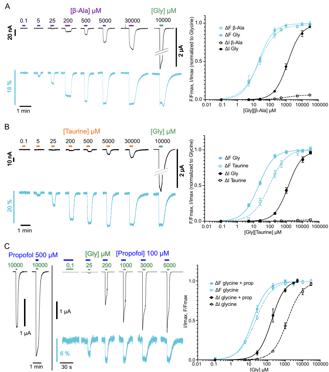
Fig. 4 | Electrophysiological and fluorescence characterization of partial-agonist ( \beta -alanine and taurine) and propofol effects on K143W/Q219C sensor on C41V GlyR. A Right panel: Representative VCF recordings on an oocyte challenged with both \beta -alanine and glycine. Left panel: representative VCF recording on oocytes under the \beta -alanine application. Right panels: the \Delta I (cyan) and \Delta F (black) curves (normalized to the glycine maximal response recorded on each individual oocyte) with mean and SEM for K143W/Q219C under glycine (solid line) and \beta -alanine (dotted line) application. The \Delta F curves for both molecules are superimposed but the efficacy of \beta -alanine to activate the receptor is lower than that of glycine ( 6.1 \pm 2.2\% of glycine maximum response in current, n = 6 ). B Right panel: Representative VCF recordings on an oocyte challenged with both taurine and
