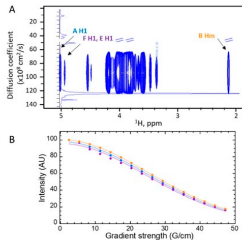
Figure 6. ^1\text{H} DOSY spectrum of the mannan polymer contained in the size exclusion chromatography FNR-B fraction obtained from the ASSN fraction (A). Experiments were recorded at 298°K. The center and width of the signals in the diffusion pseudo-dimension represent the mean and standard deviation of the diffusion coefficient at each resonance frequency, respectively. The intensity is proportional to the number of protons that contribute to the signal. All signals show the same mean and distribution ( 95 \pm 31 \times 10^{-8} \text{ cm}^2/\text{s} ), indicating that the signals pertain to the same molecule. The 1D ^1\text{H} spectrum is overlaid on the DOSY spectrum. (B) Selected diffusion curves (signal integral as a function of the gradient strength) that fit to single gaussian decays for the signals of the anomeric protons of 4-O-substituted ((A), 5 ppm, blue), unsubstituted (F) \alpha -(1,6)-mannose (4.96 ppm, purple) that overlaps with the Glc (E) H1 signal, and of GlcNAc methyl (Hm) protons ((B), 2.12 ppm, orange).
