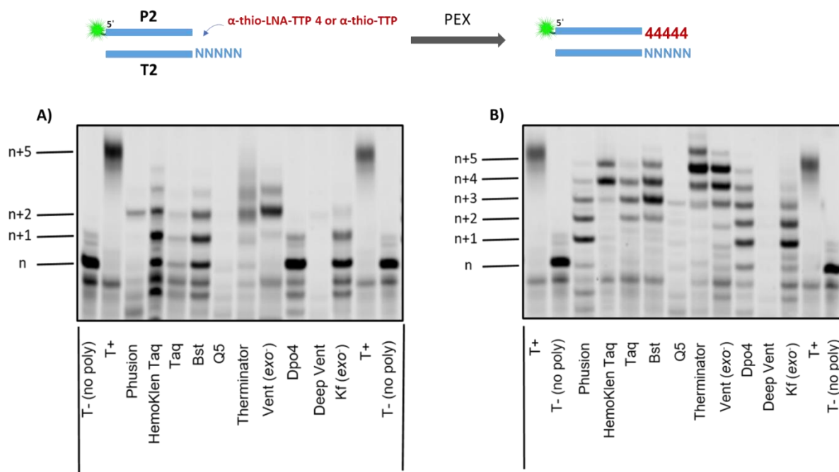
Figure 4. Gel image (PAGE 20%) analysis of products stemming from PEX reactions with primer P2 and template T2 and in the presence of various polymerases and either A) \alpha -thio-LNA-TTP 4 (200 \mu M) or B) \alpha -thio-dTTP (200 \mu M). Reactions were carried out with 10 U of polymerases and for 1h. T+ represents a positive control reaction with all four natural dNTPs, and T-(polymerase) represents a control reaction run in the absence of polymerase.
