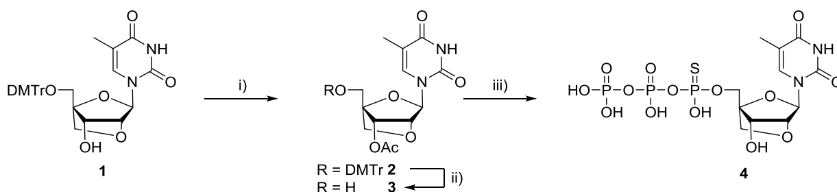
Scheme 1. Synthetic route to the modified LNA triphosphate 4 . Reagents and conditions: i) \text{Ac}_2\text{O} , DMAP, pyridine, rt, 1h, 91%; ii) TFA, DCM, rt, 1h, 80%; iii) a) 2-chloro-1,3,2-benzodioxaphosphorin-4-one, pyridine, dioxane, rt, 45 min; b) (n\text{Bu}_3\text{NH})_2 \text{H}_2\text{P}_2\text{O}_7 , DMF, n\text{Bu}_3\text{N} , rt, 45 min; c) Beaucage reagent, pyridine, rt, 30 min; d) \text{NH}_3 (aq.), rt, 2h, 31% over 4 steps.
