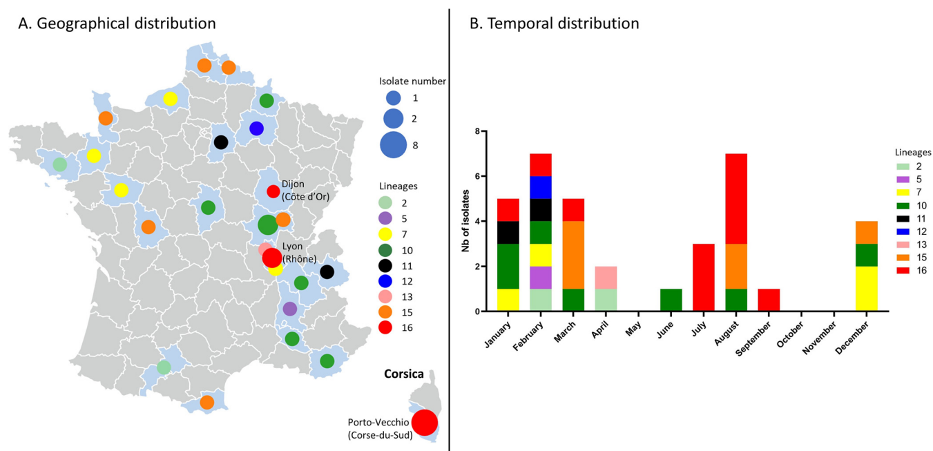
FIG 1 Geographical and temporal distribution of the 35 Y. pseudotuberculosis isolated in France in 2020. (A) Map of France with the departments. Size of the circle depends on the number of isolates. Colors of the circles depends on the isolates' lineages. (B) Number of strains per month. Colors of the squares depends on the isolates' lineages.
