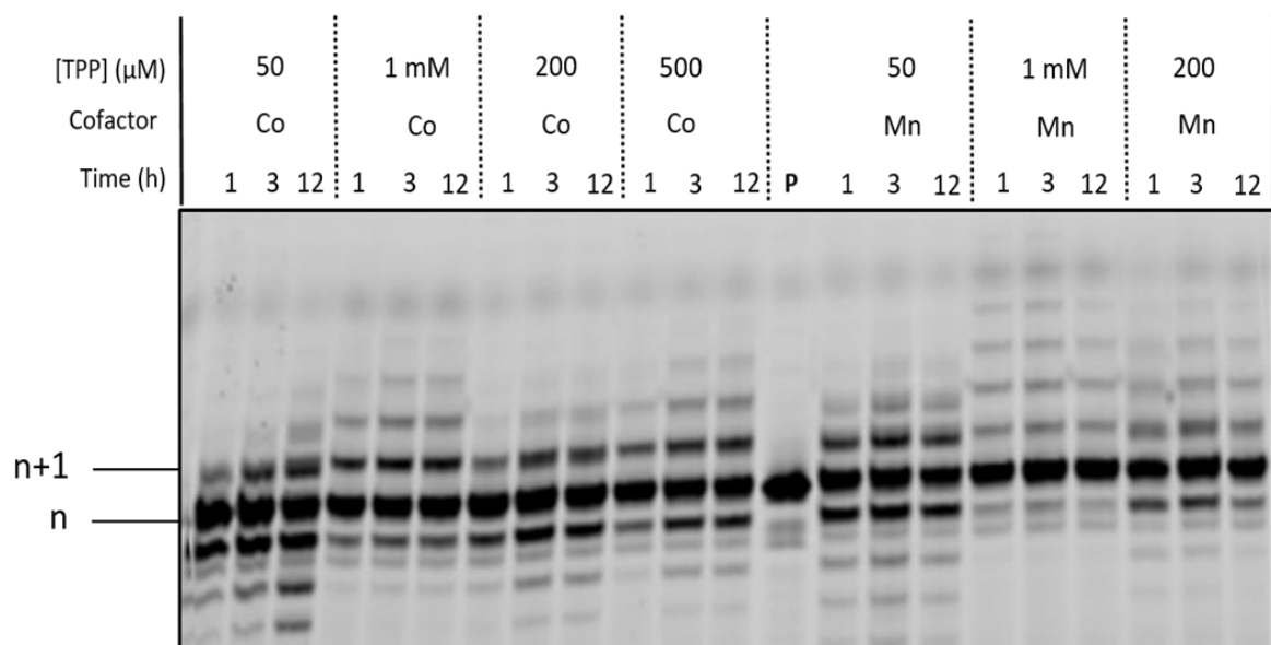
Figure 6. Gel (PAGE 20%) analysis of the products stemming from A) PEX reactions with various DNA polymerases and the P1/T1 system and B) TdT-mediated extension reactions with 5'-FAM-labelled primer P2 . PEX reaction contained natural and modified triphosphates
