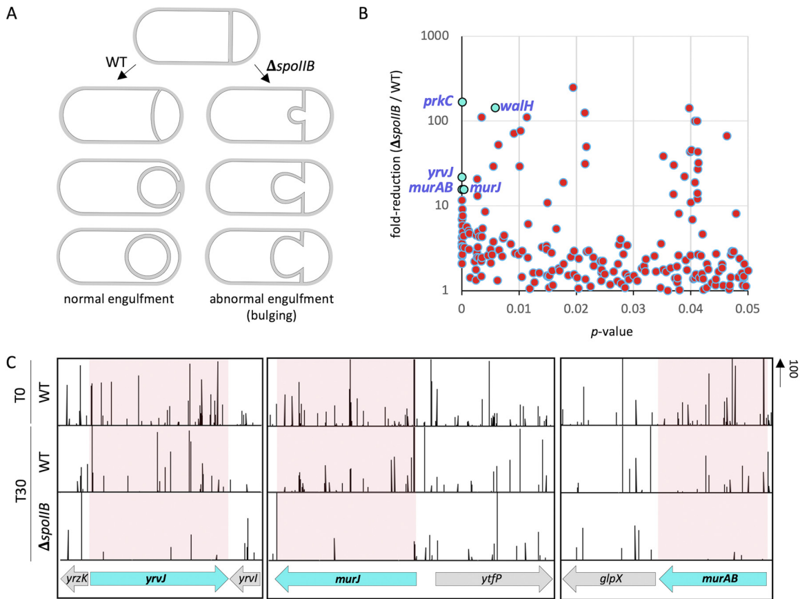
FIG 1 Tn-seq reveals genes involved in PG synthesis and hydrolysis that are important for sporulation in the absence of spoIIA . (A) Schematic representation of normal (left) and abnormal (right) engulfment in a wild-type (WT) cell and \Delta spoIIA mutant cell, respectively. In WT cells, the asymmetric septum curves and engulfment proceeds evenly around the forespore. In \Delta spoIIA cells, the asymmetric septum bulges and protrudes into the mother cell. PG is shaded in gray. (B) Scatterplot showing fold reduction of transposon insertions in \Delta spoIIA (bCR1560) relative to WT (bDR2413) cells with corresponding P values. Genes involved in PG synthesis ( murAB , murJ ) and hydrolysis ( yrvJ ) with high fold reduction in \Delta spoIIA compared to WT cells and a low P value are labeled and colored cyan. (C) Tn-seq profiles at the yrvJ , murJ , and murAB genomic loci of WT (bDR2413) and \Delta spoIIA (bCR1560) cells following 30 h of growth and sporulation in exhaustion medium. The height of the vertical lines represents the number of Tn-seq reads at each position. Shaded regions highlight the significant reduction in sequencing reads at yrvJ , murJ , and murAB loci.
