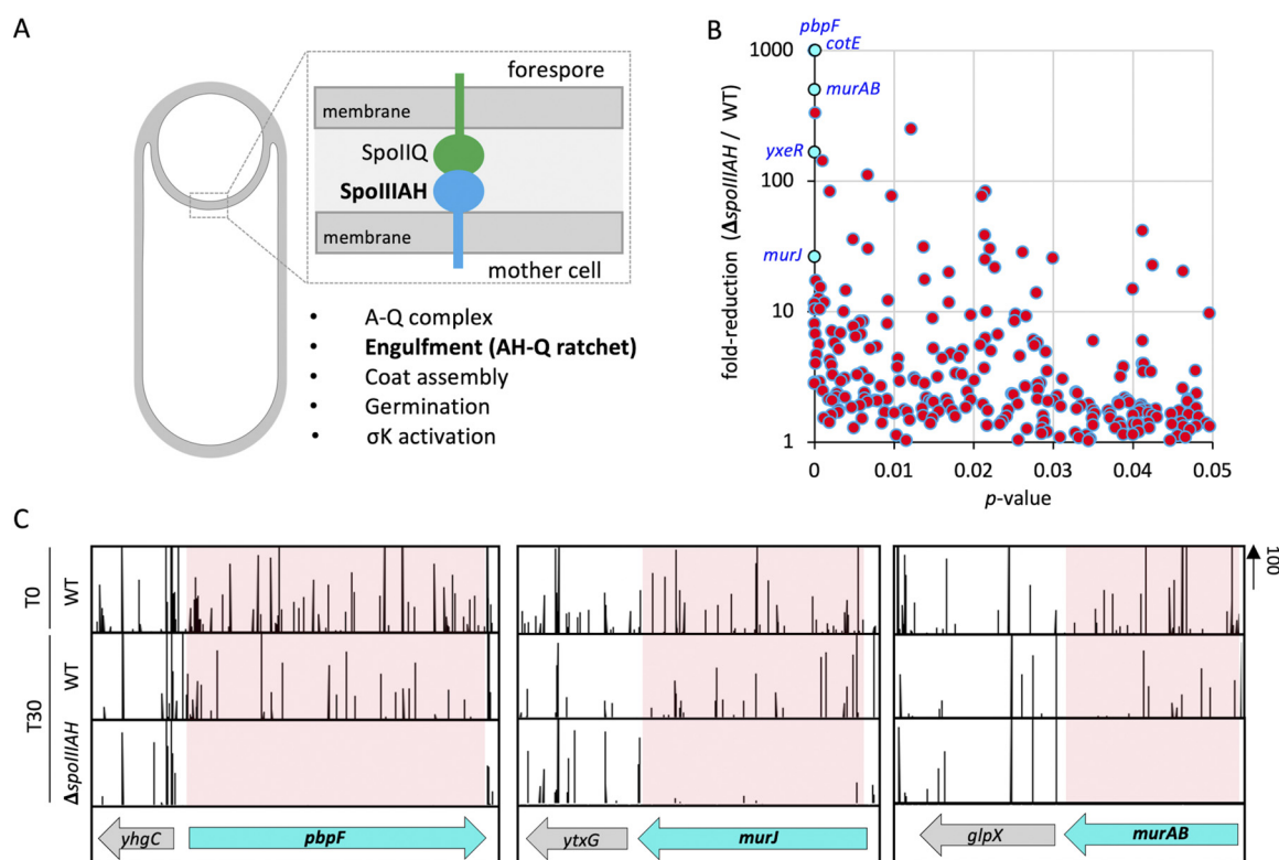
FIG 5 Tn-seq reveals genes involved in PG synthesis and hydrolysis that are important for sporulation in the absence of spoIIAH . (A) Schematic illustration of an engulfing B. subtilis cell (left), highlighting the protein interaction between SpoIIQ (green) in the forespore membrane and SpoIIAH (blue) in the engulfing mother cell membrane. The SpoIIQ-SpoIIAH interaction is required for efficient A-Q complex formation, engulfment, coat assembly, germination, and \sigma^K activation. PG is shaded in light gray. (B) Scatterplot showing fold-reduction of transposon insertions in \Delta spoIIAH (bCR1117) relative to WT (bDR2413) cells with corresponding P values. Genes related to peptidoglycan synthesis ( murAB , murJ , pbpF ), metabolism ( yxgR ) and coat assembly ( cotE ) with high fold reduction in \Delta spoIIAH compared to WT cells and a low P value are labeled and colored cyan. (C) Tn-seq profiles at the pbpF , murJ , and murAB genomic loci of WT (bDR2413) and \Delta spoIIAH (bCR1117) cells, following 30 h of growth and sporulation in exhaustion medium. Height of vertical lines represents number of Tn-seq reads at each position. Shaded regions highlight the significant reduction in sequencing reads at the pbpF , murJ , and murAB loci.
