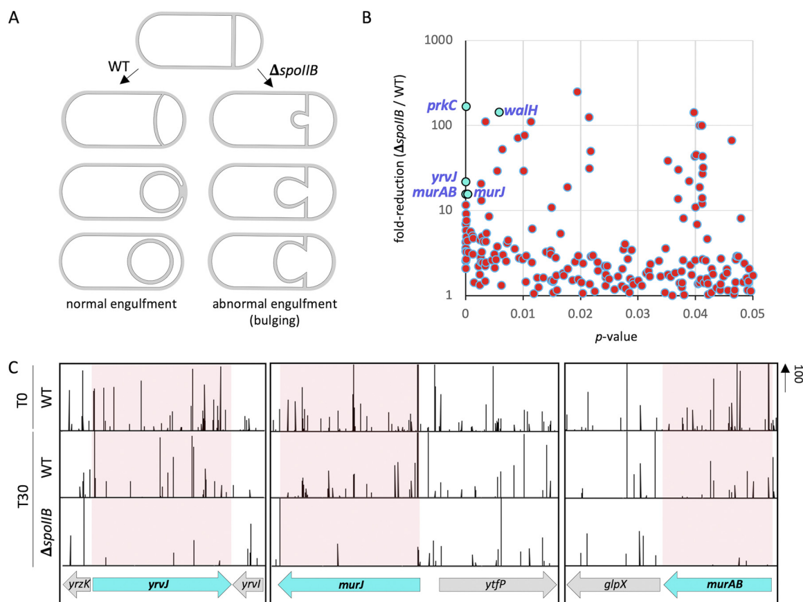
FIG 1 Tn-seq reveals genes involved in PG synthesis and hydrolysis that are important for sporulation in the absence of spoIIIB . (A) Schematic representation of normal (left) and abnormal (right) engulfment in a wild-type (WT) cell and \Delta spoIIIB mutant cell, respectively. In WT cells, the asymmetric septum curves and engulfment proceeds evenly around the forespore. In \Delta spoIIIB cells, the asymmetric septum bulges and protrudes into the mother cell. PG is shaded in gray. (B) Scatterplot showing fold reduction of transposon insertions in \Delta spoIIIB (bCR1560) relative to WT (bDR2413) cells with corresponding P values. Genes involved in PG synthesis ( murAB , murJ ) and hydrolysis ( yrvJ ) with high fold reduction in \Delta spoIIIB compared to WT cells and a low P value are labeled and colored cyan. (C) Tn-seq profiles at the yrvJ , murJ , and murAB genomic loci of WT (bDR2413) and \Delta spoIIIB (bCR1560) cells following 30 h of growth and sporulation in exhaustion medium. The height of the vertical lines represents the number of Tn-seq reads at each position. Shaded regions highlight the significant reduction in sequencing reads at yrvJ , murJ , and murAB loci.
