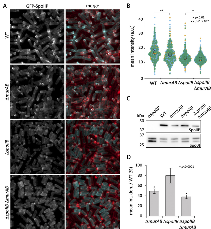
FIG 4 GFP-SpoIIP localization in the absence of spoIIB and murAB . (A) GFP-SpoIIP localization and (B) distribution of GFP-SpoIIP mean fluorescence intensity (a.u.) in the wild-type (WT) (bHC544), \Delta murAB (bHC545), \Delta spoIIB (bHC546), and \Delta spoIIB \Delta murAB (bHC547) strains at 2.5 h after onset of sporulation (T2.5). GFP signal is false-colored cyan in merged images. Cell membranes were visualized with TMA-DPH fluorescent membrane dye and are false-colored red in merged images. Scale bar = 2 \mu m . Panel B is a superplot with totals of 489, 528, 645, and 694 cells for the WT, \Delta murAB , \Delta spoIIB , and \Delta spoIIB \Delta murAB strains, respectively. *, P < 0.01 , and **, P < 1 \times 10^{-8} , by Kolmogorov-Smirnov test performed on the combined distribution of replicates ( n = 3 ). The Welch's t test was also performed on the means with P < 0.05 for the WT versus the \Delta murAB mutant and the \Delta spoIIB mutant versus the \Delta spoIIB \Delta murAB mutant. (C) Immunoblot analysis of SpoIIP in the \Delta spoIIP (bHC550), WT (bDR2413), \Delta murAB (bAT73), \Delta spoIIB (bCR1560) and \Delta spoIIB \Delta murAB (bHC203) strains at T2.5. SpoIIP was detected using anti-SpoIIP antibodies. Spo0J was used as a loading control and was detected using anti-Spo0J antibodies. (D) Mean integrated density of SpoIIP bands relative to the WT as detected by immunoblot analysis in panel C. Error bars represent the SD from three biological replicates. *, P < 0.0001 by Student's t test.
