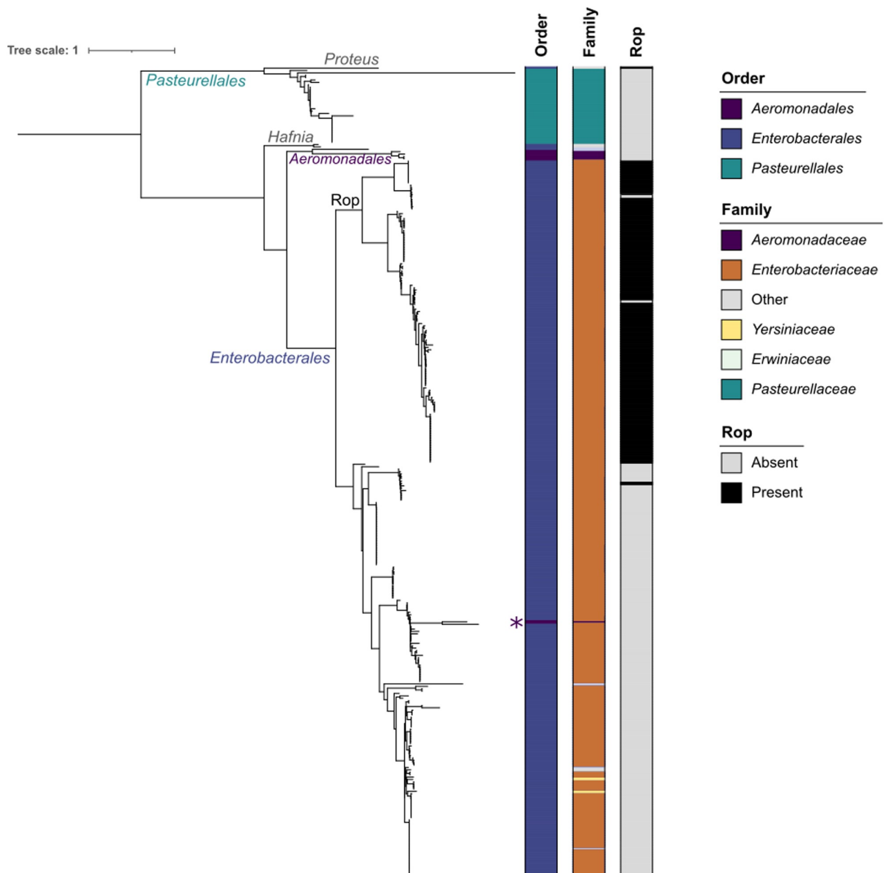
Fig 5. Phylogenetic tree of the 339 MOB PS/HEN relaxases. The colors of the columns at the right of the tree indicate, from the left to the right, the host Order, the host Family and the presence or absence of the rop gene in the plasmid. The asterisk next to the first column at the right of the tree represents the only relaxase clustered with plasmids of other Order. The phylogenetic tree was inferred following the best-fit model, JTT+F+I+G4.
