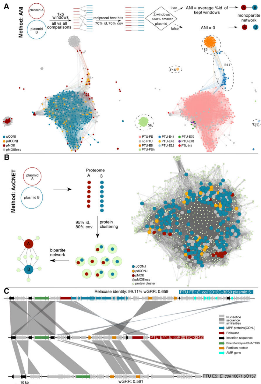
Fig. 7. (A) Graphical representation of the algorithm used for the ANI calculation: each plasmid nucleotide sequence was divided into overlapped 1 kb windows and for each plasmid pair, all stretches were compared. ANI scores were obtained by averaging the percentage of identity of all considered windows with identity and coverage >70%, whenever the sum of windows covered at least the 50% of the smallest plasmid in the pair. ANI scores different from 0 were represented as edges connecting the members of the plasmid pair (nodes) in the ANI network. ANI similarity network of the MOB F12 plasmid family from E. coli and Shigella spp: The genomic relatedness of 353 transmissible MOB F12 plasmids hosted in E. coli and Shigella spp., and 140 MOBless plasmids belonging to the same PTUs was estimated by pairwise ANI calculations. At the left, nodes are colored by their mobility type, and at the right, by their PTU. “no PTU” means nonassigned PTU. In the right panel, PTUs that are separated from the main group (PTU-F E ) are surrounded by a circle. (B) Graphical representation of the method used for the plasmid proteome network analysis: the protein set of all plasmids to be compared is clustered at 95% amino acid identity and 80% alignment coverage. The homologous protein clusters and their corresponding plasmids are the two kinds of nodes represented in the network and edges connect both types whenever a plasmid contains a member in a given protein cluster. Proteome network of the PTU-F E plasmids. The proteins of 250 PTU-F E plasmids were clustered at 95% identity and 80% coverage. Whenever a plasmid has a member in a protein cluster, an edge is linking them. Homologous protein clusters present in a single plasmid were removed from the figure. Plasmids are colored by their mobility type. (C) Comparison between selected PTU-F E , PTU-E 41 , and PTU-E 5 plasmids. Plotted using GenoPlotR v.0.8.10 (Guy et al. 2010), based on Blastn analysis of the plasmid nucleotide sequences ( e -value < 10 -4 and alignment length > 1000 bp). Comparison between a pCONJ (blue), a pMOB (red), and a pMOBless plasmid (gray). For clarity, we only represent best bidirectional regions of homology larger than 1 kb with more than 50% identity. Genes involved in the plasmid mobility (T4SS and relaxase[s]), antimicrobial resistance (AMR), plasmid partitioning, pathogenicity, and insertion sequences are highlighted.
