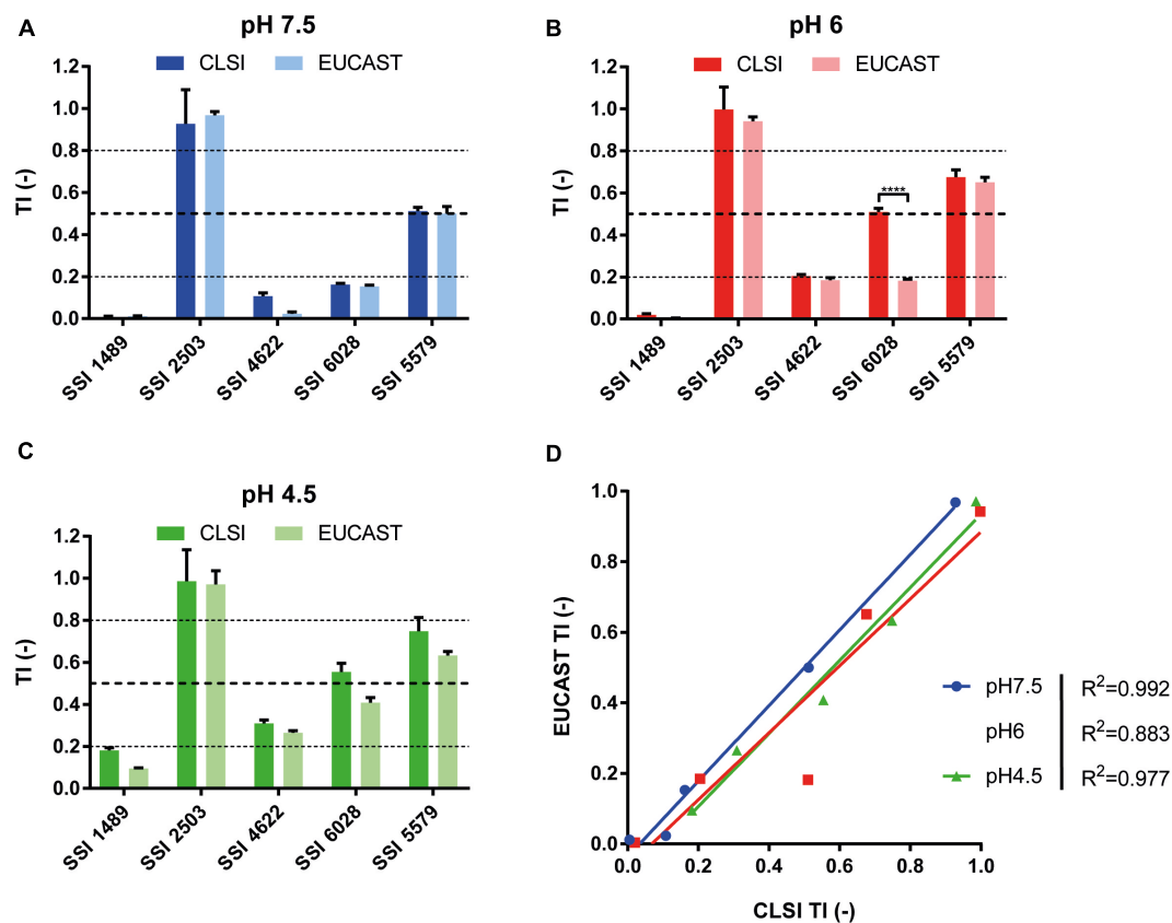
FIGURE 1 | Comparison of CLSI and EUCAST protocols for the identification of tolerant isolates. Comparison was performed at pHs 7.5, 6.0, and 4.5 (A–C, respectively) to assess the pH effect upon tolerance as stated by Marr et al. (1999). (D) Represents the correlation between both approaches with the respective R^2 corresponding to each tested pH (Two-tailed Pearson correlation, confidence interval = 95%). Each bar corresponds to the mean of biological duplicates. Statistical significance was calculated using Sidak's multiple comparison tests (two-way ANOVA, 95% confidence interval). P -values: <0.0001 (****).
