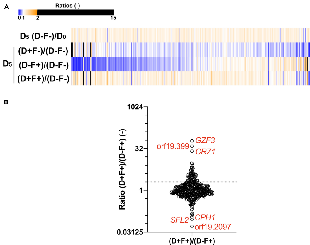
FIGURE 3 | Comparisons of the population of the 572-Tet-inducible OE strains collection pool after 5 days of enrichment. (A) The heatmap represents the comparison between the cultures at day 5 (D 5 ) and the initial population (D 0 ), in presence (F+) or absence (F-) of FLC (32 μg/ml), and in the presence (D+) or absence (D-) of 100 μg/ml Dox. Each line represents the mean relative count ratio of biological duplicates. The heatmap is filtered based on the [D 5 (D+F+)/D 5 (D-F+)] comparison. (B) Enrichment of specific Tet-dependent OE strains in the presence of FLC with and without Dox. The dotted line represents a 2-fold threshold enrichment between FLC exposed cells in the absence and presence of Dox. Y-axis is in log 2 scale. Detailed data can be found in Supplementary File S2 .
