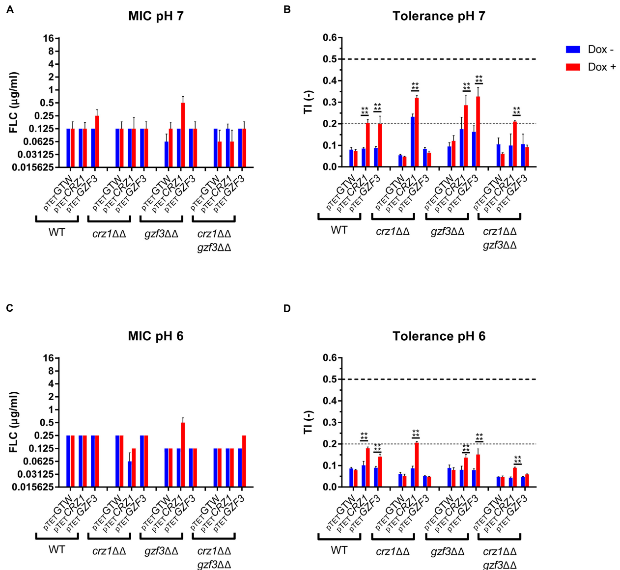
FIGURE 6 | Susceptibility profile of the CRZ1 and GZF3 mutants overexpressing either CRZ1 , GZF3 . (A,C) Susceptibility to FLC is represented as the modal MIC value with standard deviation calculated on the mean MIC of all replicates. (B,D) Tolerance profile of the mutant strains. The mean TI and standard deviations are represented. Horizontal dashed lines represent the lower threshold of tolerance (TI = 2), and the upper limit of susceptibility (TI = 0.5) as described by EUCAST. Each data set represents the mean (or mode) of biological duplicates. Statistical significances (B,D) were estimated using Sidak's multiple comparison tests (two-way ANOVA, 95% confidence interval) between Dox- and Dox+ conditions in the same mutants set. P -values: (****) \leq 0.0001 . Supplementary Table S1 lists correspondence between genotype and strain number.
