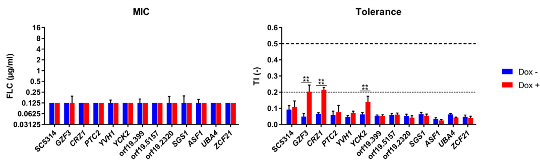
FIGURE 5 | Susceptibility profiles of selected Tet-inducible strains in the presence Dox. Susceptibility profiles were performed at pH 6, in a range of FLC concentrations (0–16 \mu\text{g/ml} ), in the presence (Dox+) or absence (Dox-) of doxycycline at 100 \mu\text{g/ml} and complemented with 1 mM \text{FeCl}_3 . FLC susceptibility was presented by their modal MIC value (left panel) and TIs at 8 \mu\text{g/ml} FLC (right panel). Standard deviations of the MIC values were calculated based on the mean MIC of each sample. The horizontal dashed line represents the lower threshold of tolerance (TI = 0.2) and the limit of susceptibility (TI = 0.5) as defined by EUCAST. Each bar is representative of biological triplicates. Statistical significance was determined using Sidak's multiple comparison tests (Two-way ANOVA, Confidence interval = 95 %). P -values: (****) \leq 0.0001 .
