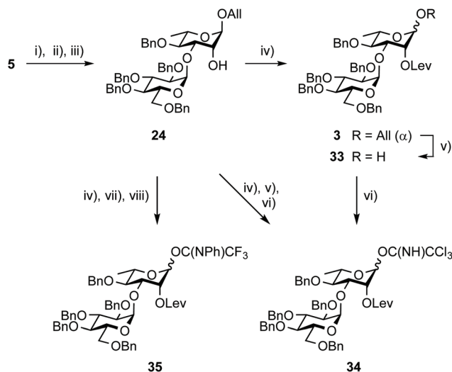
Scheme 7 Synthesis of donors EA from diol 5 and tetra-benzyl glucosyl donors 21 or 22 . (i) MeC(OMe) 3 , PTSA-H 2 O, MeCN, rt then 80% aq. AcOH, 0 °C; (iii) TfOH, DMF, 4 Å MS, DCM, –78 °C to rt; (iii) MeONa, MeOH/DCM, from 21 (1.15 equiv.), 88% (over two steps) and from 22 (1.3 equiv.), 79% (over three steps); (iv) LevOH, EDC, DMAP, DCM, 90% (30 g scale); (v) [Ir(COD){PCH 3 (C 6 H 5 ) 2 ] + PF 6 – , THF, then I 2 , THF/H 2 O, 85% (29 g scale); (vi) CCl 3 CN, DBU, DCE, –5 °C, 93% (23 g scale), also from 24 , 67%, (42 g scale, 3 steps) together with 25 (30%); (vii) PdCl 2 , DCM/H 2 O then I 2 , THF, 50 °C; (viii) PTFACl, K 2 CO 3 , acetone, 90% (34 g scale, 3 steps).
