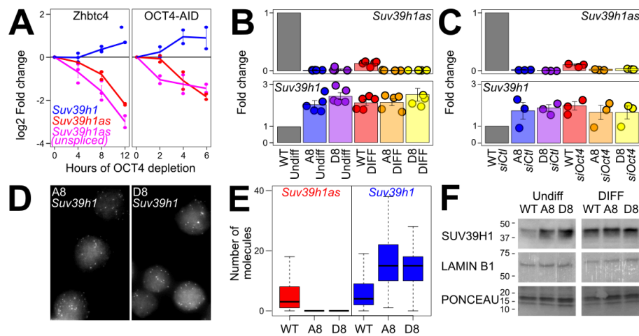
1 2 3 Figure 3: OCT4 represses Suv39h1 via Suv39h1as . (A) Log 2 expression fold change of Suv39h1 (blue), Suv39h1as (red) 4 and unspliced Suv39h1as (magenta) upon OCT4 depletion in ZHBTC4 (left) and OCT4-AID (right) cells. The 5 X-axis shows the number of hours of treatment with Dox (ZHBTC4) and IAA (OCT4-AID). Two biological replicates 6 per cell line and time-point are shown. The global effect of the treatments was assessed by comparing all time 7 points together against untreated cells with a t test ( p < 0.02 for both ZHBTC4 and OCT4-AID). (B) Expression fold 8 change of Suv39h1as (top) and Suv39h1 (bottom) in WT and Suv39h1as -mutant cells (A8 and D8) cultured in 9 undifferentiated or differentiating conditions (3 days without LIF). Values were normalized to Tbp . Each dot 10 represents an independent replicate and the bar and error bars the corresponding means and standard errors. 11 The increase of Suv39h1 in each clone versus WT cells was compared with a t test ( p = 0.011 and 0.0016 for A8 12 and D8, respectively). (C) Expression fold change of Suv39h1as (top) and Suv39h1 (bottom) in WT and Suv39h1as - 13 mutant cells (A8 and D8) knocked-down with either control or Oct4 -targeted siRNAs. Values were normalized to 14 Tbp . Each dot represents an independent replicate and the bar and error bars the corresponding means and 15 standard errors. The increase of Suv39h1 expression upon OCT4 knock-down was assessed against control siRNAs 16 with a t test ( p = 0.027 in WT cells). (D) Representative sm-FISH images of Suv39h1 in A8 and D8 cells (WT cells 17 presented in Fig.2D). Differences in the frequency of active transcription sites were assessed with a Chi 2 test 18 ( p < 10^{-10} for both clones against WT cells) (E) Boxplots (median; 25-75% percentiles; error bars) showing the 19 number of Suv39h1as (red) or Suv39h1 (blue) diffusible molecules counted in WT ( n = 358 ) or mutant cells (A8, 20 n = 289 ; D8, n = 270 ). Differences in the number of Suv39h1 molecules were assessed with a Mann-Whitney test 21 ( p < 10^{-15} for both clones against WT cells). (F) Representative Western-Blot of SUV39H1, LAMIN B1 and 22 corresponding Ponceau for WT and mutant cells (A8 and D8) in undifferentiated and differentiating (3 days 23 without LIF) conditions. On the left of each image is indicated the protein scale in kDa.
