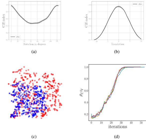
Fig. 12: C 3 I scores are shown for registering rotated and translated 2D Gaussian data in (a) and (b) respectively. The target set (red) and the source set (blue) for point-set registration are illustrated in (c). In (d), C 3 I values during the successive iterations of CPD algorithm is plotted for five distinct registration experiments.
