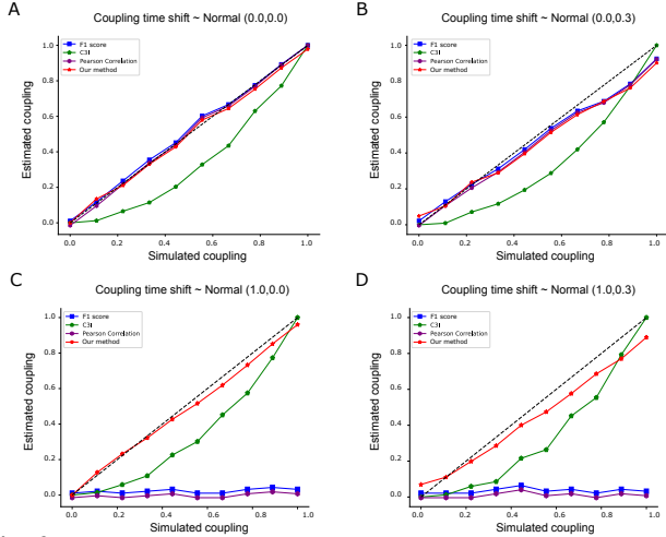
Fig. 2: Robustness of correlation metrics to different coupling time shifts. Our statistical method (red) is compared with standard correlation metrics (Pearson correlation coefficient (purple), F1 score (blue) and C3I (green)) for increasing simulated coupling level and different time shifts (A- t_{shift} \sim \mathcal{N}(\mu_s = 0, \sigma_s = 0) , B- t_{shift} \sim \mathcal{N}(0, 0.3) , C- t_{shift} \sim \mathcal{N}(1, 0) , and D- t_{shift} \sim \mathcal{N}(1, 0.3) .)
