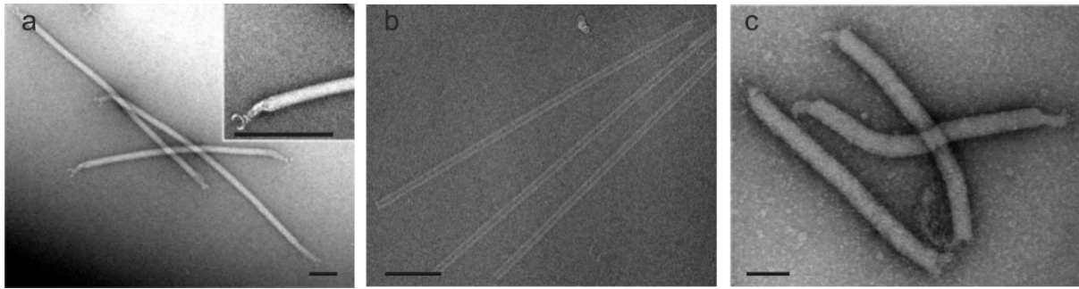
Figure 3. Electron micrographs of archaeal viruses with filamentous morphologies. (a) AFV1, Acidianus filamentous virus 1, the inset displays the terminal structure; (b) SIRV2, Sulfolobus islandicus rod-shaped virus 2; and (c) PFV1, Pyrobaculum filamentous virus 1. Negative stain with uranyl acetate, except for SIRV2, which is in vitreous ice. Bars, 100 nm. Image modified from Prangishvili, D., Bamford, D.H., Forterre, P., Iranzo, J., Koonin, E.V., and Krupovic, M. (2017). The enigmatic archaeal virosphere. Nature reviews Microbiology 15, 724-739.
