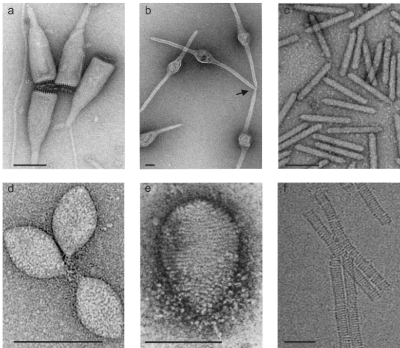
Figure 1. Electron micrographs of archaeal viruses with particular morphologies. (a) ABV, Acidianus bottle-shaped virus; (b) ATV, Acidianus two-tailed virus, the arrow indicates virion tails which underwent extracellular development; (c) APBV1, Aeropyrum pernix bacilliform virus 1; (d) SSV1, Sulfolobus spindle-shaped virus 1; (e) SNDV, Sulfolobus neozealandicus droplet-shaped virus, and (f) ACV, Aeropyrum coil-shaped virus. Negative stain with uranyl acetate, except for ACV, which is in vitreous ice. Bars, 100 nm. Image modified from Prangishvili, D., Bamford, D.H., Forterre, P., Iranzo, J., Koonin, E.V., and Krupovic, M. (2017). The enigmatic archaeal virosphere. Nature reviews Microbiology 15, 724-739.
