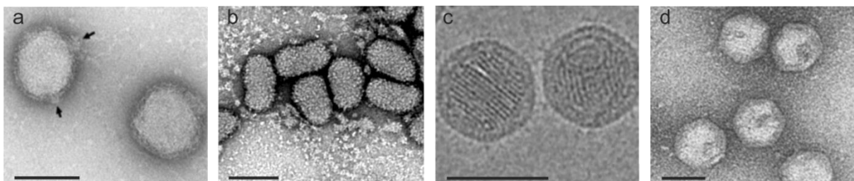
Figure 2. Electron micrographs of archaeal viruses with spherical morphologies. (a) PSV1, Pyrobaculum spherical virus 1, the arrows indicate spherical protrusions; (b) SEV1, Sulfolobus ellipsoid virus 1; (c) SPV1, Sulfolobus polyhedral virus 1; and (d) STIV, Sulfolobus turreted icosahedral virus. Negative stain with uranyl acetate. Bars, 100 nm. Image modified from Prangishvili, D., Bamford, D.H., Forterre, P., Iranzo, J., Koonin, E.V., and Krupovic, M. (2017). The enigmatic archaeal virosphere. Nature reviews Microbiology 15, 724-739. SEV1 image is courtesy of L. Huang.
