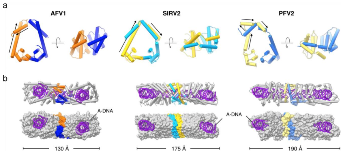
Figure 4. Virion organization of the filamentous viruses AFV1, SIRV2 and PFV2. (a) Comparison of the MCP dimer (asymmetric unit) of AFV1 (left), SIRV2 (centre) and PFV2 (right). The MCP1 of AFV1, SIRV2 and PFV2 are colored in orange, gold and yellow, respectively. The MCP2 of AFV1, SIRV2 and PFV2 are coloured in blue, cyan and light blue, respectively. The N-terminal helices of MCP1 in AFV1, SIRV2 and PFV2 are marked with black arrows. (b) Wrapping of A-form DNA in AFV1, SIRV2 and PFV2. One MCP dimer is colored as in (a), other four dimers are coloured in gray. Proteins are shown in ribbon representation (top) and as surfaces (bottom). Image reproduced from Wang, F., Baquero, D.P., Su, Z., Osinski, T., Prangishvili, D., Egelman, E.H., and Krupovic, M. (2020). Structure of a filamentous virus uncovers familial ties within the archaeal virosphere. Virus evolution 6, veaa023.
