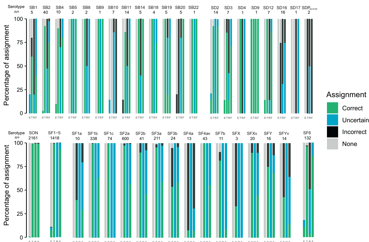
Fig. 9 Graphical representation of the in silico serotyping results for 3861 Shigella “routine” isolates according to each serotype prediction tool.
