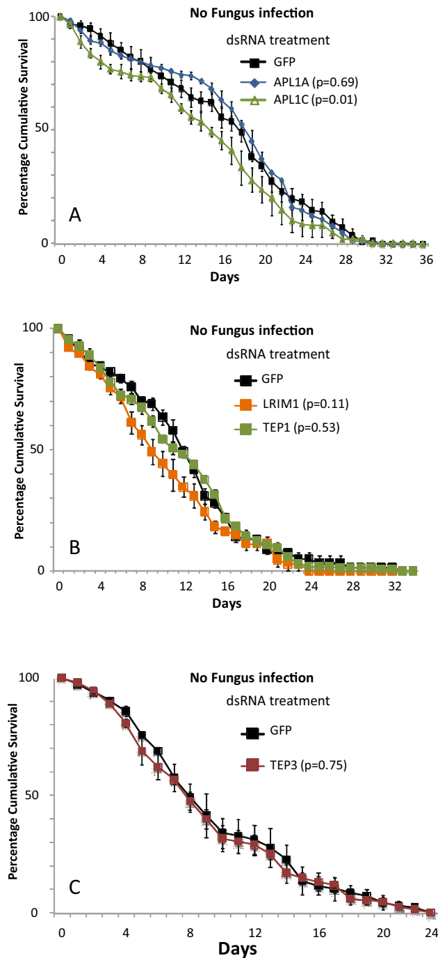
Figure 6. APL1C silencing in male A. coluzzii causes increased mortality. The graphs illustrate mortality curves of male mosquitoes after gene silencing without infection (A) Silencing of APL1A and APL1C genes expression, (B) Silencing of LRIM1 and TEP1 gene expression, (C) Silencing of TEP3 gene expression. p -values obtained from Cox Regression are mentioned in brackets with the respective gene. Error bars represent the variability between three independent biological replicates. For each tested gene, 150 (50 per replicate) mosquitoes were used for all three biological replicates.
