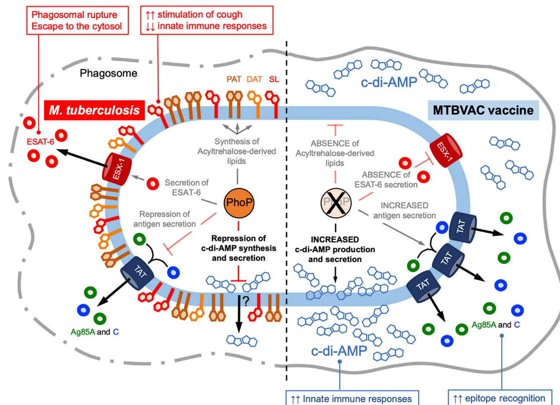
Figure 6. Schematic representation of the PhoPR-related phenotypes in M. tuberculosis (left side) and MTBVAC (right side) in the context of the macrophage environment
