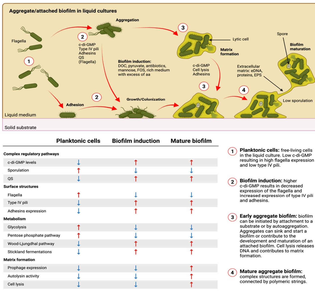
Figure 2. Model for C. difficile aggregate/attached biofilm formation in vitro. The first step toward biofilm formation is either attachment of the cells to a surface or cellular aggregation. In both cases a shift in surface structures controlled by rising c-di-GMP levels results in the replacement of the flagella by T4P and adhesins (collagen and fibronectin binding proteins). Autolysin-mediated cell lysis is likely the main mechanism contributing to the formation of the extracellular matrix by releasing chromosomal DNA and cellular proteins in the medium, and exopolysaccharides may be synthesized and contribute to the matrix. Quorum sensing may induce prophage lysis that would also contribute to the biofilm matrix. Furthermore, c-di-GMP levels remain relatively high, ensuring consistent T4P and adhesins expression. C. difficile biofilm formation is characterized by a metabolic shift from glycolysis and the pentose phosphate pathway to the Stickland fermentation pathways and the Wood-Ljungdhal pathway, which are less efficient at producing energy. The table summarizes information about the main mechanisms involved in biofilm formation. Up-regulated mechanisms are indicated by the red upward arrows and the down-regulated mechanisms are indicated by the blue downward arrows. Abbreviations: aa: amino acids; QS: quorum sensing; eDNA: extracellular DNA; EPS: exopolysaccharides; DOC: deoxycholate; FOS: fructooligosaccharides.
