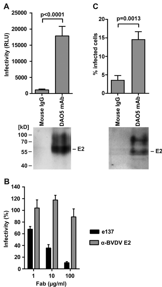
FIG 5 More than one conformation of the Ig-like domain was observed on both HCVpp and HCVcc infectious particles. (A) Concentrated HCVpp were immunocaptured using Immuno tubes. After removing unbound material, the captured particles were analyzed by SDS-PAGE, followed by immunoblotting to detect E2 (lower panel). The presence of captured infectious HCVpp was determined by overnight incubation with Huh7 cells in suspension. The cells were then transferred into tissue culture dishes, and infectivity levels were determined 48 h later by measuring luciferase activity, shown as relative light units (RLU) (upper panel). (B) DAO5-captured particles were incubated with Huh7 cells as described for panel A in the presence of e137 Fab or control anti-bovine viral diarrhea virus (BVDV) E2 Fab at the indicated concentrations. Infectivity levels were determined as described above and are shown as the percent infectivity in the absence of Fab. (C) Concentrated HCVcc were immunocaptured as described for panel A. After removing unbound material, captured particles were analyzed by SDS-PAGE followed by immunoblotting to detect E2 (lower panel). The presence of captured infectious HCVcc was determined by overnight incubation with Huh7 cells in suspension. The cells were then transferred into tissue culture dishes, and the number of infected cells was determined after 72 h by flow cytometry after labeling with anti-N55A MAb 9E10 (upper panel). Experiments were performed at least in triplicate, and results shown are means \pm standard deviations. The P values (panel A and C) were calculated using an unpaired t test.
