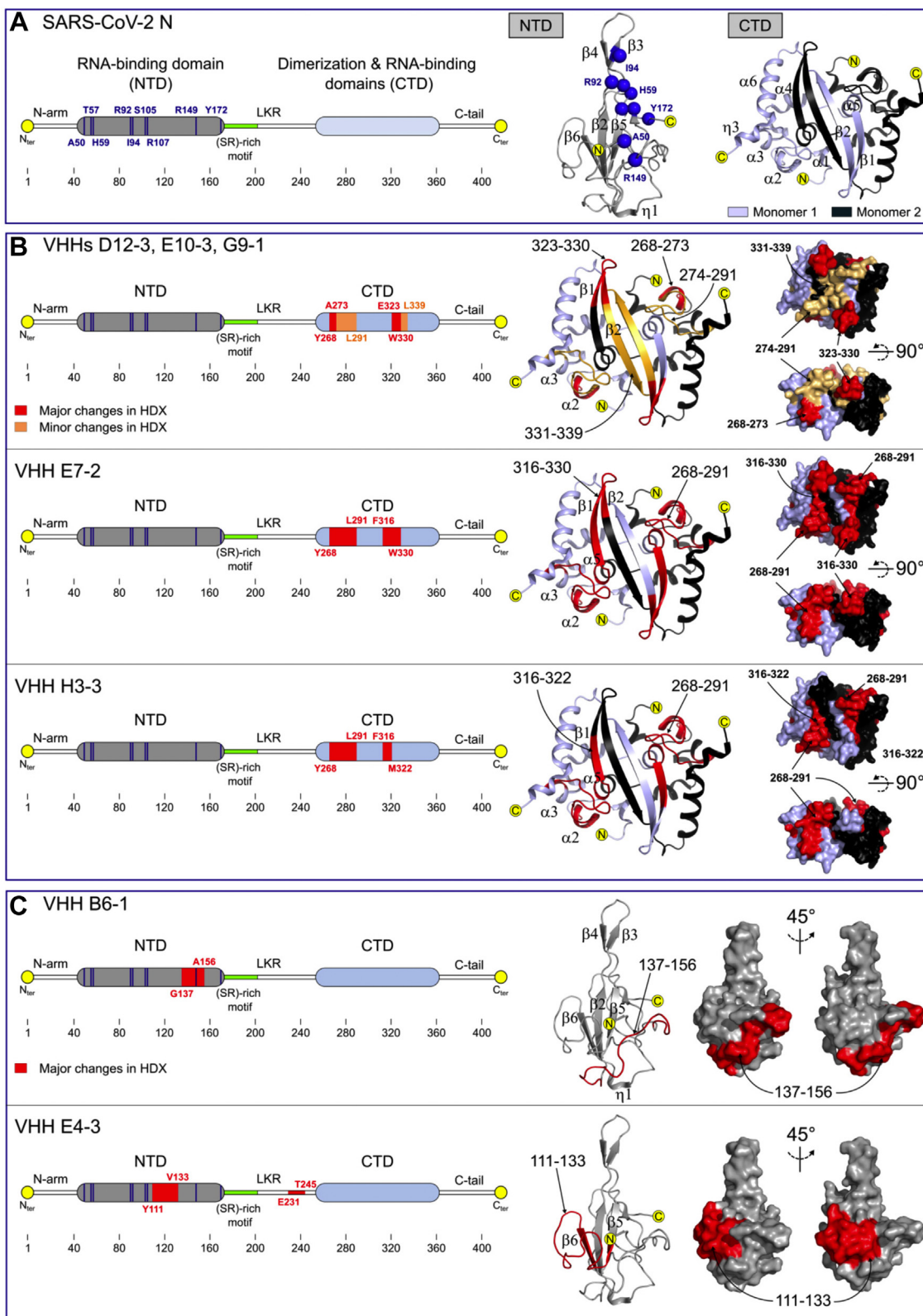
Figure 4. Comparison of the VHH epitopes mapped by HDX-MS. A, linear representation (left) of full-length SARS-CoV-2 N with NTD in gray and CTD in light blue. The cartoon representations of the NTD domain (pdb # 7CDZ) and the CTD dimer (pdb # 7CE0) are shown on the right panel, with one CTD monomer colored light blue and the other colored black. The RNA-binding residues identified by NMR are also reported on the linear (left, blue bars) and the cartoon representations of the NTD domain (right, blue spheres). B and C, comparison of the epitopes identified in the CTD (B) and the NTD (C) domains by HDX-MS. Red and orange patches correspond to regions where major and minor reductions in solvent accessibility were observed upon VHH binding. HDX-MS results are mapped onto the cartoon and surface representations of the NTD and CTD domains.
