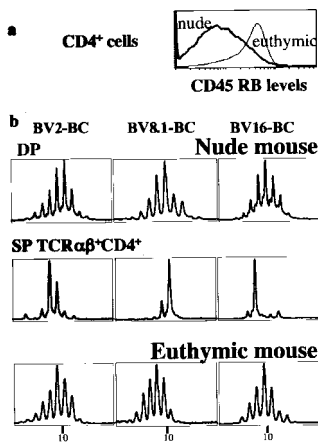
Figure 3. Exploration of the memory phenotype and of the TCR \beta repertoire of MLN \alpha\beta^+ CD4 ^+ cells of nude and euthymic mice. (a) MLN CD4 ^+ cells from a nude mouse express the phenotype of memory cells, in contrast with comparable cells from an euthymic mouse. Cells were triply labeled with anti-TCR \beta , anti-CD4, and anti-CD45RB mAbs. (b) The TCR \beta repertoire of MLN DP cells from a nude mouse shows the gaussian-like profile characteristic of polyclonal populations (top), whereas that of SP CD4 ^+ cells is oligoclonal (middle), in contrast with that of comparable cells from an euthymic mouse (bottom).
