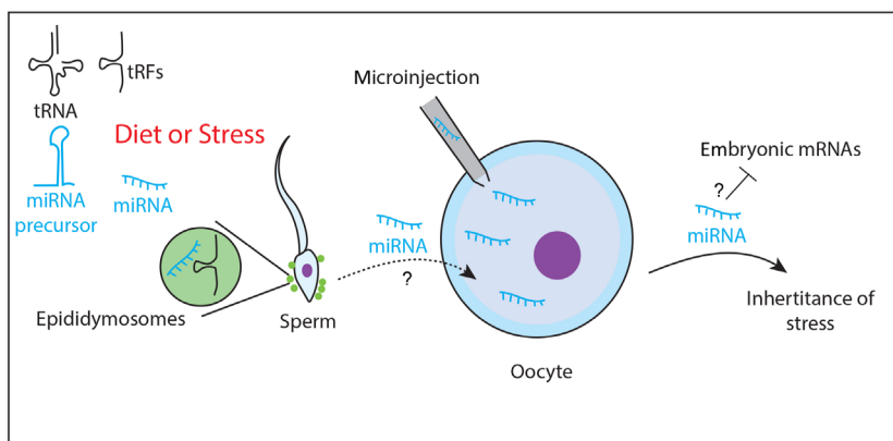
Fig. 3. Paternal inheritance of miRNAs in the mouse. Metabolic changes or different types of stress alter the small RNA cargoes loaded into mature mouse sperm. Diet-induced tRNA fragmentation results in high production of tRFs loaded into mature sperm through epididymosomes vesicles. These vesicles might also transport miRNAs induced by stress. The microinjection of miRNAs extracted from mature sperm produced by animals subjected to stresses recapitulates the stress-induced phenotypes in subsequent generations. It is unclear whether the miRNA cargoes loaded into mature sperm can effectively regulate embryonic mRNAs after fertilization.
