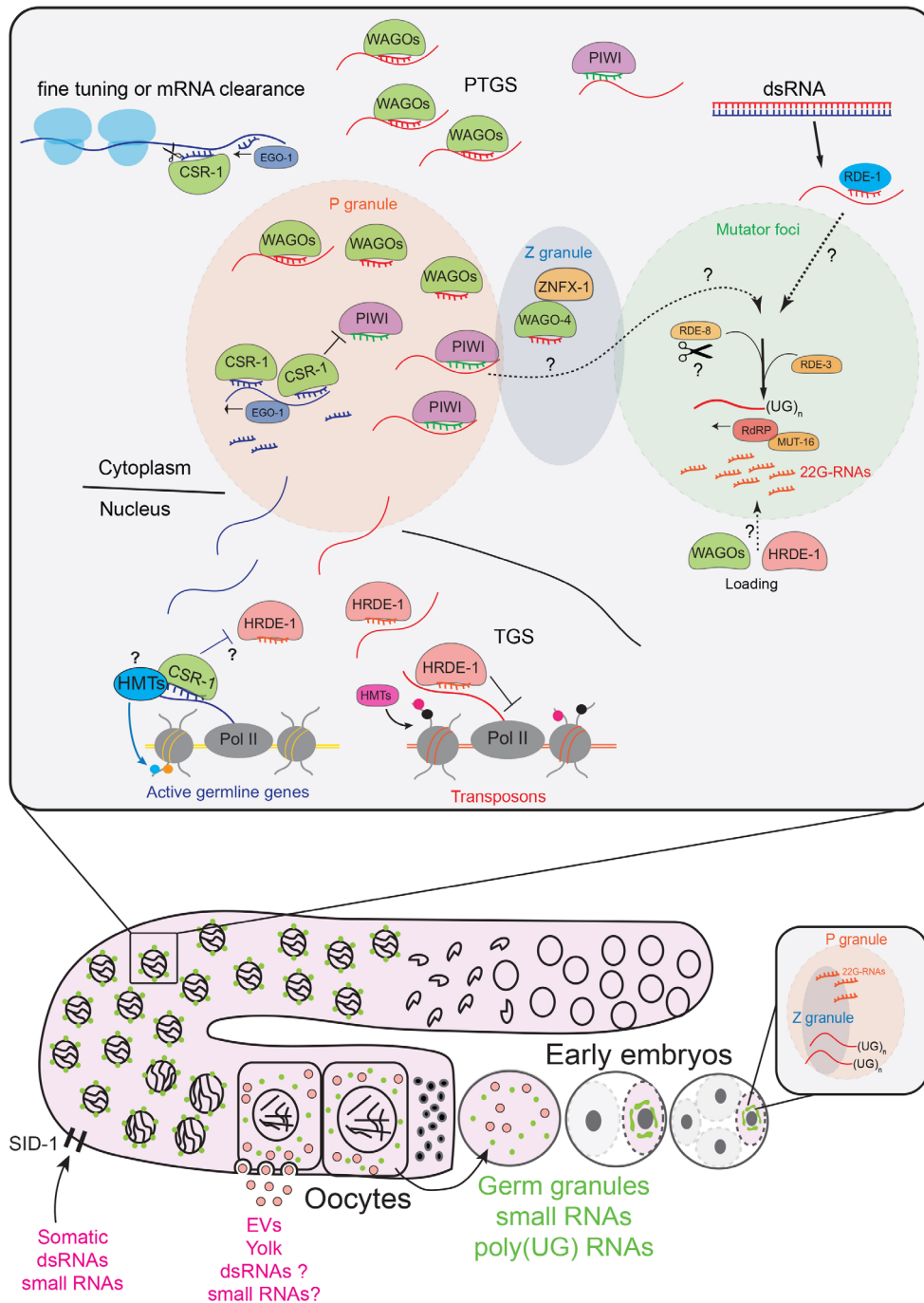
Fig. 2. Schematic of the different endogenous germline small RNA pathways and their inheritance in C. elegans . Most of the Argonaute proteins localize to germ granules, phase-separated condensates surrounding the nuclear membrane in the germline of C. elegans . Three different condensates characterize germ granules (P granules, Z granules, and mutator foci). The P granules contain most of the WAGOs, PIWI, and CSR-1 proteins. The Z granules contain factors involved in heritable RNAi. The mutator foci include most of the enzymes required for the biogenesis of 22G-RNAs triggered by dsRNAs or piRNAs. The 22G-RNAs derived from active germline genes are produced by the RdRP EGO-1 and are loaded into the Argonaute CSR-1. These CSR-1 22G-RNAs can protect germline mRNAs from piRNA silencing and promote the degradation of the complementary mRNAs in the cytosol through the CSR-1 catalytic activity. CSR-1 can also bind nascent transcripts and prevent HRDE-1 nuclear silencing. Most of the germline 22G-RNAs and pUGylated mRNAs are transmitted to the embryos inside the germ granules. Somatic 22G-RNAs and dsRNAs are transmitted to the germline through the dsRNA receptor SID-1 or possibly through EVs carrying yolk protein from the intestine to the oocytes.
