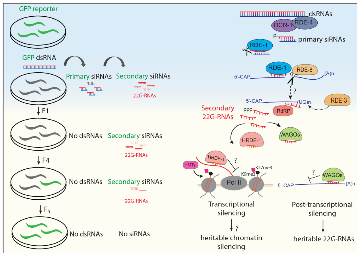
Fig. 1. Schematic of the inheritance of C. elegans RNAi. The exposure to dsRNAs targeting a fluorescent GFP sequence leads to the inactivation of the GFP reporter (green and gray worms). The GFP reporter remains silenced even in subsequent generations that are not exposed to dsRNAs. The production of primary siRNAs generated by Dicer (DCR-1) and its cofactor RDE-4 are loaded into the Argonaute RDE-1. The catalytic activity of RDE-1 serves to remove one of the strands of the double-stranded siRNA. The targeting of the complementary sequence by RDE-1 leads to the recruitment of the endonuclease RDE-8 and subsequently to the pUGylation of the cleaved mRNAs. pUGylated mRNAs become the substrate for the RdRP, which generates secondary single-stranded 5' triphosphorylated small RNAs called 22G-RNAs. The 22G-RNAs are loaded into downstream WAGO proteins, the effector Argonautes that trigger post-transcriptional and transcriptional silencing. Such silencing persists for multiple generations and correlates with the presence of inherited 22G-RNAs and pUGylated mRNAs. The nuclear Argonaute HRDE-1 also triggers heritable histone PTMs.
