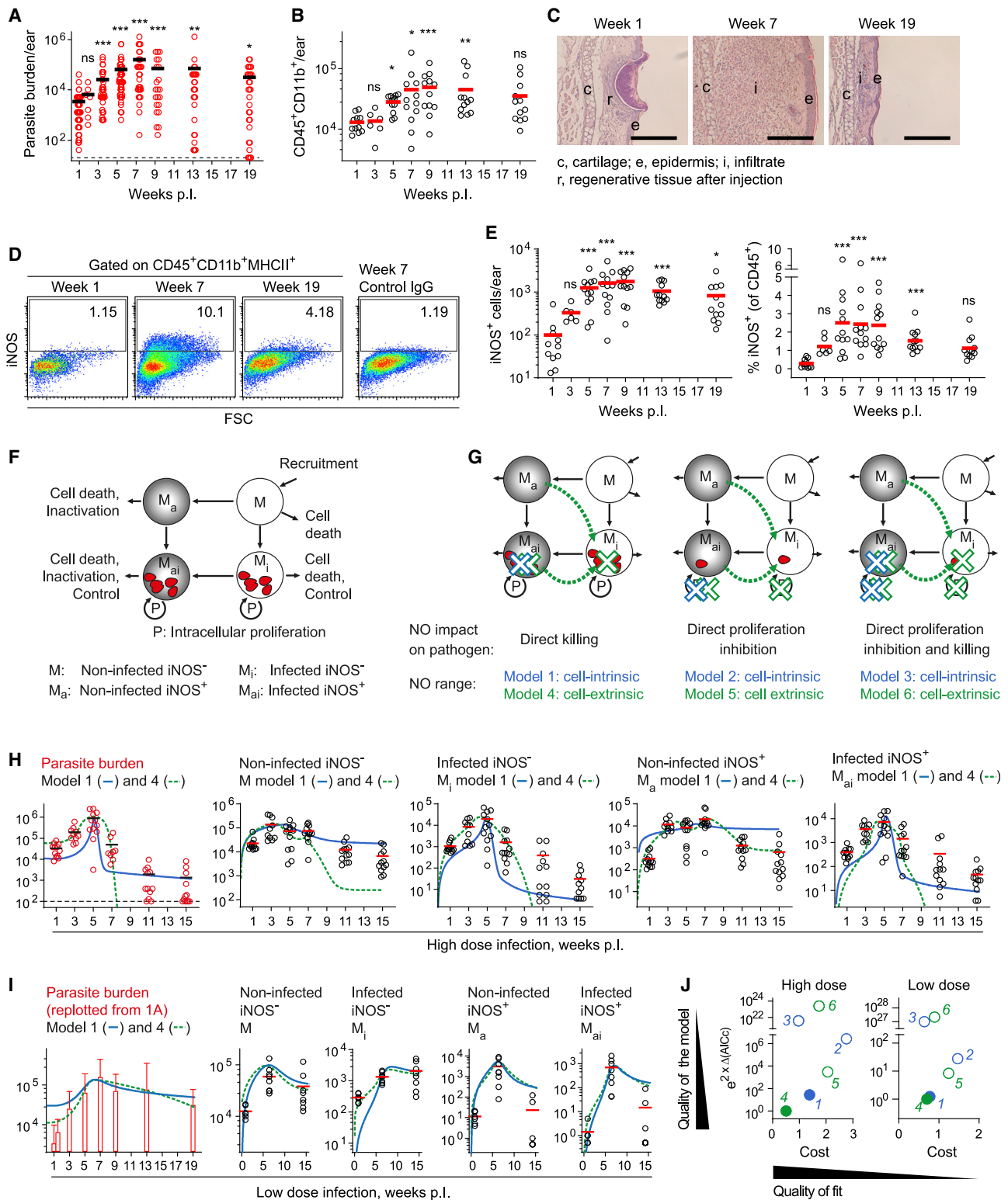
Figure 1. Ordinary differential equation-based modeling of L. major high- and low-dose infection
