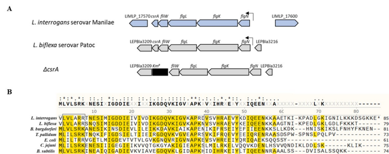
Fig 1. csrA operon in Leptospira spp. (A) A genetic organization of csrA in Leptospira spp. The arrangement of the genes in the csrA operon in L. interrogans , L. biflexa , and L. biflexa \Delta csrA are shown. (B) The alignment of the amino acid sequences of CsrA in L. biflexa serovar Patoc and L. interrogans serovar Manilae strains used in this study was performed in comparison with CsrA from other bacteria. (*) represents conserved amino acid and the square boxes indicate conserved residues that are important for RNA binding in E. coli [62]. Sequences highlighted in yellow indicate the conserved residues.
