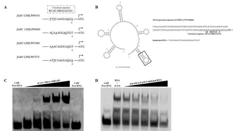
Fig 9. L. interrogans CsrA regulated flaB expression. (A) Analysis of flaB 5' untranslated regions of L. interrogans serovar Manilae. The genes and distances to the start codon are indicated. Underlined letters represent mismatched nucleotides compared to the consensus sequence. (B) Secondary structure of 120-nucleotide 5' untranslated region of LIMLP07475 (FlaB4) was predicted using MFOLD [64]. The putative CsrA binding site is shown and the start codon (ATG) is indicated in bold letters. The sequences of the synthesized 5' biotinylated RNA of LIMLP_07475 is shown. (C) Electrophoretic mobility shift assay (EMSA), 1 nM biotinylated RNA of LIMLP_07475 was incubated with different concentrations of L. interrogans rCsrA. The reaction solution was subjected to 10% native PAGE, transferred to a nylon membrane, probed with HRP-conjugated streptavidin, and detected for chemiluminescent signal after the detection reagent was added. (D) Competitive EMSA, biotinylated RNA of LIMLP_07475 and rCsrA concentration were fixed at 1 nM and 800 nM, respectively. Unlabeled LIMLP_07475 was added in the reaction concentration range from 0.8 nM to 8 μM.
