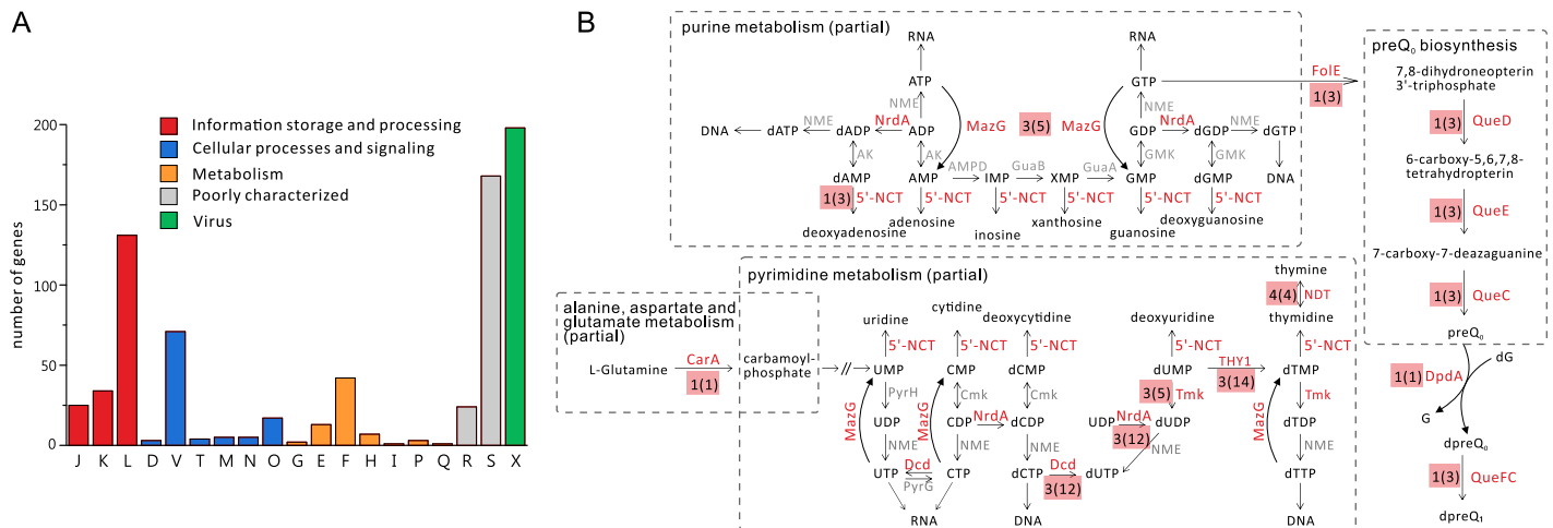
Fig 4. Classification of genes encoded by arTVs. (A) Classification of arTV genes into arCOG functional categories. The homologous gene shared by viruses in the same species is counted as one. The letters represent the following: J, translation, ribosomal structure and biogenesis; K, transcription; L, replication, recombination and repair; D, cell cycle control, cell division, chromosome partitioning; V, defense mechanisms; T, signal transduction mechanisms; M, cell wall/membrane/envelope biogenesis; N, cell motility; O, posttranslational modification, protein turnover, chaperons; G, carbohydrate transport and metabolism; E, amino acid transport and metabolism; F, nucleotide transport and metabolism; H, coenzyme transport and metabolism; I, lipid transport and metabolism; P, inorganic ion transport and metabolism; Q, secondary metabolites biosynthesis, transport and catabolism; R, general function prediction only; S, function unknown; X, virus related. (B) Schematic showing nucleotide-related (partial) metabolic pathways, with a particular enzyme indicated for each reaction. Enzymes that are found encoded by arTVs are in red, otherwise in gray. The number of virus families that harbor the enzyme is indicated next to the enzyme name, with the number of virus species shown in parentheses. NrdA: RnR, MazG: NTP pyrophosphatase, 5'-NCT: 5'-deoxyribonucleotidase, CarA: CP synthase small subunit, Dcd: dCTP deaminase, Tmk: thymidylate kinase, THY1: thymidylate synthase thyX, NDT: nucleoside deoxyribosyltransferase, Fole: GTP cyclohydrolase I, QueC: queuosine biosynthesis protein, QueD: 6-pyruvoyl tetrahydropterin synthase, QueE: 7-carboxy-7-deazaguanine synthase, DpdA: paralog of queuine tRNA-ribosyltransferase, QueFC: NADPH-dependent 7-cyano-7-deazaguanine reductase. See S3 and S5 Tables for individual genes classification. arCOG, archaeal clusters of orthologous gene; arTV, archaeal tailed virus; CP, carbamoylphosphate; RnR, ribonucleotide diphosphate reductase.
