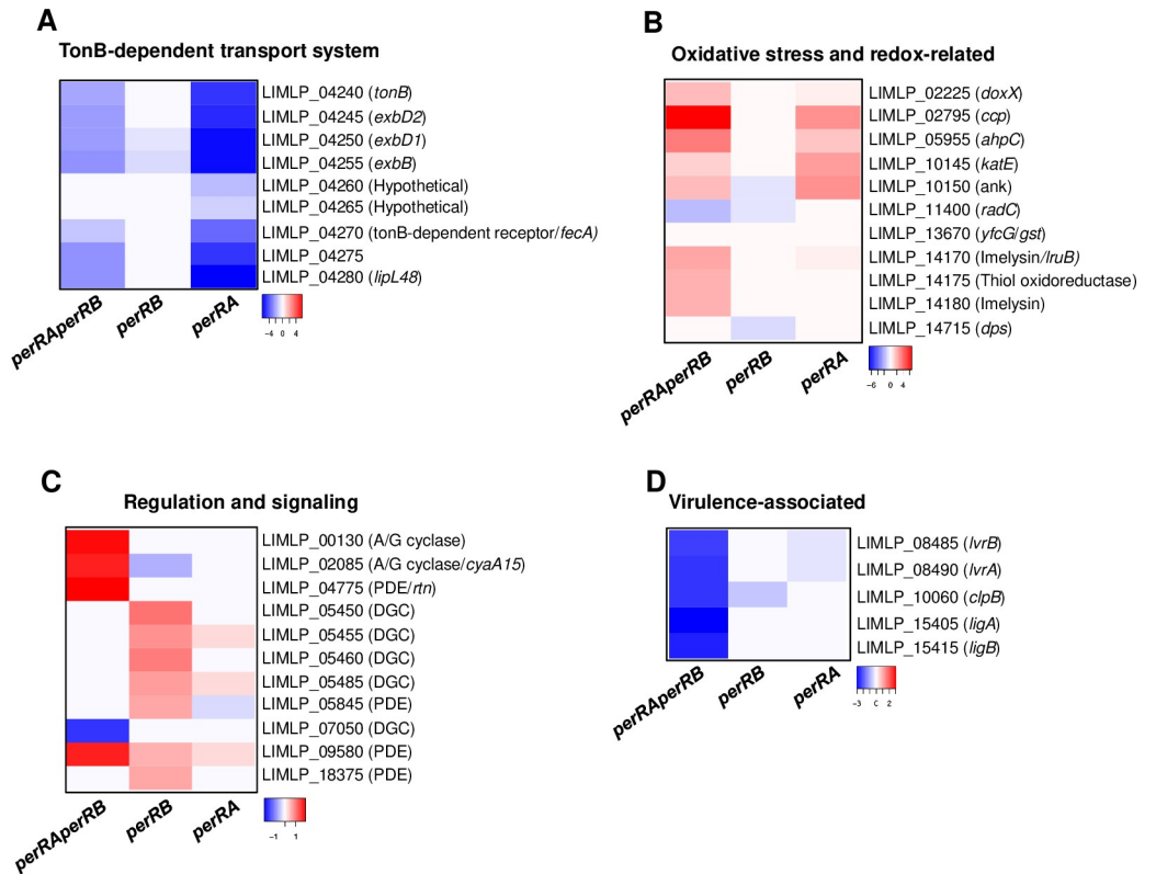
Fig 9. Comparison of differential gene expression in the double perRAperRB mutant with that in the single perRA and perRB mutants. Expression of selected genes of the TonB-dependent transport cluster (A), involved in oxidative stress and redox homeostasis (B), in regulation and signaling (C), and in virulence (D) determined by RNASeq in the double perRAperRB mutant was compared to those in the single perRA mutant determined by Zavala-Alvarado et al. [19] and single perRB mutant (as determined in this study). Differential expression in each mutant strain was normalized with that in the WT strain. Gene names are indicated on the right. The Heat Map color from blue to red indicates low to high \text{Log}_2\text{FC} .
