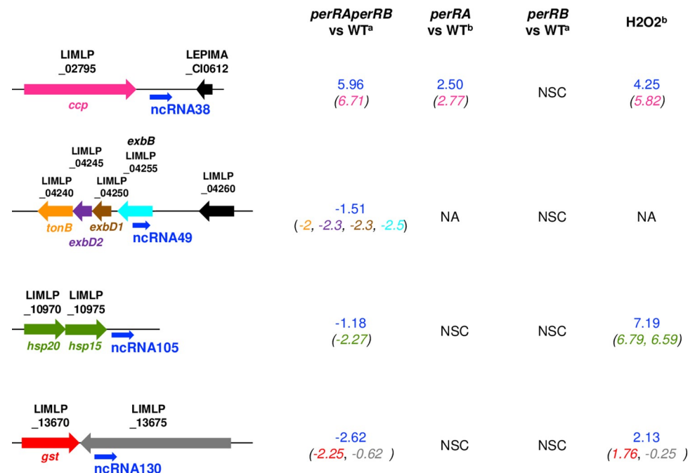
Fig 10. Non-coding RNAs expression in the double perRAperRB mutant. Differential expression of selected ncRNAs (LepncRNA38, 49, 105, and 130) in the perRAperRB mutant (determined in this study) ( a ) was compared to those in the single perRA mutant, as determined by Zavala-Alvarado et al. [19] ( b ), in the single perRB mutant (determined by this study) ( c ), and upon exposure to 1 mM H 2 O 2 for 1h00 as determined by Zavala-Alvarado et al. [19] ( b ). The location of the ncRNAs LepncRNA38, 49, 105, and 130 were represented schematically with the adjacent or overlapping ORFs. The values indicate the Log 2 FC of ncRNAs expression normalized with that in WT. The respective expression of these ORFs (Log 2 FC) are indicated into parenthesis with the same color as their representation in the cartoon. NSC, non-significantly changed; NA, non-applicable.
