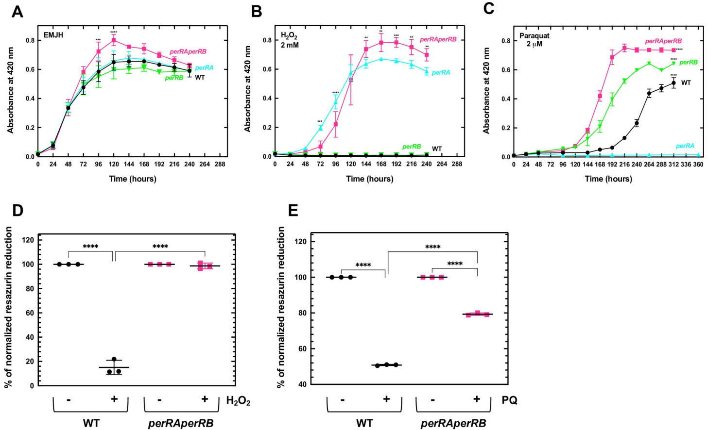
Fig 6. Effect of concomitant inactivation of perA and perB on Leptospira growth in the presence of ROS. L. interrogans WT (black circles), the single perA mutant (cyan triangles), the single perB mutants (green inverted triangles) or the double perRAperRB mutant (pink squares) were cultivated in EMJH medium in the absence (A), or in the presence of 2 mM H 2 O 2 (B) or 2 μM paraquat (C). Growth was assessed by measure of absorbance at 420 nm and the data are means and standard errors of three independent biological replicates. In panel A, statistical significance between the perRAperRB mutant and the other strains was determined by Two-way Anova test (***, p-value<0.0008; ****, p-value<0.0001). In panel B, statistical significance between the perRA and the perRAperRB mutants was determined by two-way Anova test (**, p-value<0.008; ***, p-value<0.0005; ****, p-value<0.0001). In panel C, two-way Anova test indicated that differences between WT, perRB mutant, and perRAperRB mutant were significant from 144 h (****, p-value<0.0001). Quantitative survival tests were performed by incubating exponentially growing WT (black circles) and double perRAperRB mutant (pink squares) with 5 mM H 2 O 2 for 30 min (D) or 100 μM paraquat for 60 min (E). Resazurin reduction was determined as described in the Materials and Methods section. Data are means and standard errors of three independent biological replicates. Statistical significance was determined by a One-way Anova test (****, p-value<0.0001).
