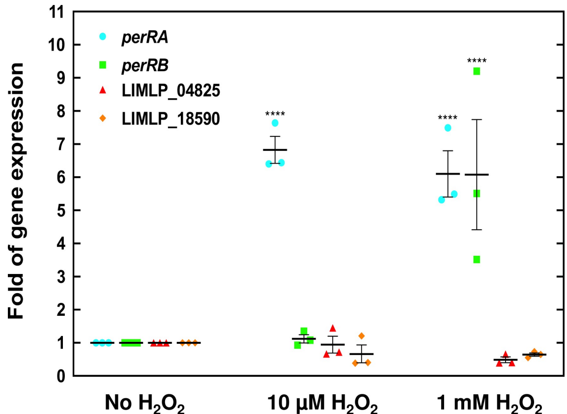
Fig 4. Increased perRA and perRB expression upon exposure to hydrogen peroxide. Exponentially growing L. interrogans were incubated in the absence or presence of 10 \mu M (for 30 min.) or 1 mM H 2 O 2 (for 60 min.) and the expression of perRA (cyan circles), perRB (green squares), LIMLP_04825 (red triangles) and LIMLP_18590 (orange diamonds) was measured by RT-qPCR as described in the Materials and Methods section using flaB as reference gene. Gene expression was normalized by that in untreated samples. Data are the means and standard errors of three independent biological replicates. Two-way Anova test indicated statistical significance in comparison with untreated samples (****, p-values < 0.0001).
