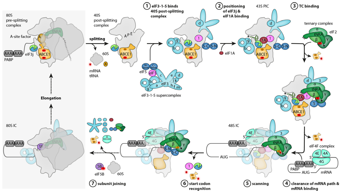
Figure 8. Role of ABC1 in eukaryotic translation initiation.
