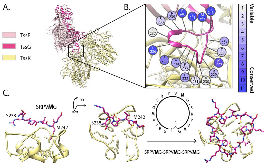
FIG 4 Biomimetic inhibitor in silico design. (A) EAEC wedge complex (PDB ID 6GLY). The box indicates the position of TssG foot 1, the template used to design the inhibitor. (B) The residue conservation of TssG foot 1 calculated from EAEC variants was used together with other indicators, such as coevolution, to select the biomimetic candidate segment (see Materials and Methods). (C) A 6-residue peptide of foot 1 (from S238 to G243) was used to generate a cyclic peptide that mimics foot 1 in its interaction with TssK trimer.
