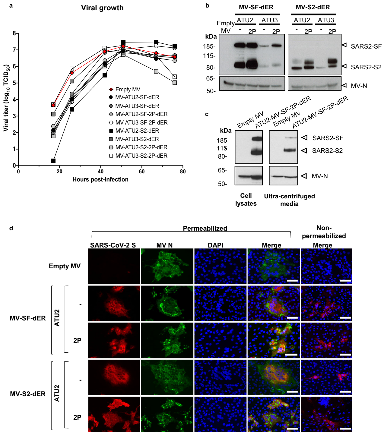
Fig. 2 Characterization of S-expressing rMVs. a Growth kinetics of rMV constructs used to infect Vero cells at an MOI of 0.1. Cell-associated virus titers are indicated in TCID 50 /ml. b Western blot analysis of SARS-CoV-2 S protein in cell lysates of Vero cells infected with the rMVs expressing SF-dER or S2-dER from either ATU2 or ATU3, with or without the 2P mutation. c Western blot analysis of ultracentrifuged media and cell lysates of Vero infected with rMV-ATU2-SF-2P-dER. d Immunofluorescence staining of Vero cells infected with the indicated rMVs 24 h after infection. Permeabilized or non-permeabilized cells were stained for S (red), MV N (green) and nuclei (blue); \times 20 magnification (scale bar, 50 \mu m). The experiments shown were conducted using two or three biologically independent Vero cell batches.
