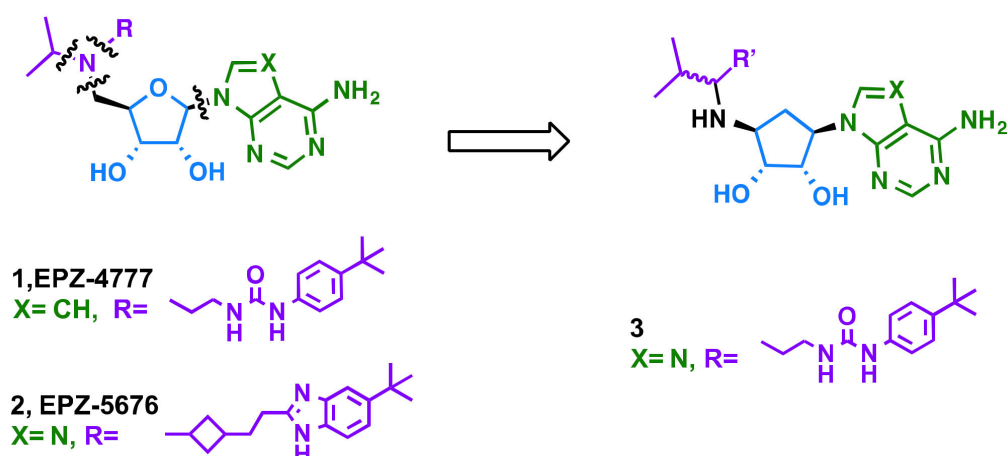
Figure 1. Chemical strategy: the metabolic sensitive points were replaced by more stable features. In green the adenine scaffold, in blue the sugar, and in purple the side chain specific of DOT1L inhibition.
