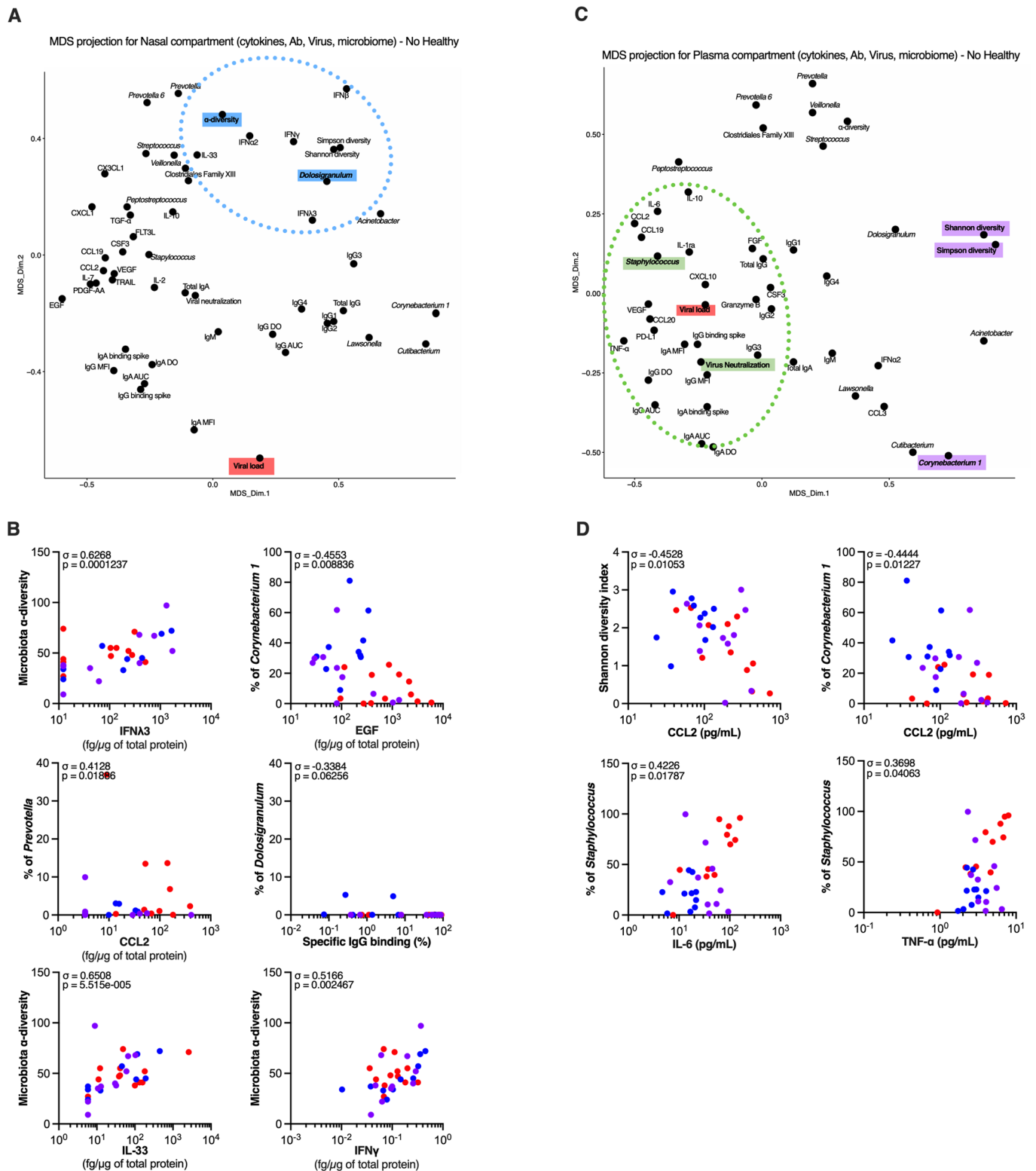
Extended Data Fig. 9 | Impact of healthy donors on microbiome analysis of integrated SARS-CoV-2 immune responses. Multidimensional scaling (MDS) projection for (a) nasopharyngeal compartment (nasal cytokines, nasal antibodies, nasal virus neutralization, nasal viral load and nasal microbiome) and (c) systemic compartment (plasma cytokines, plasma antibodies, serum virus neutralization, blood viral load and nasal microbiome). The dotted lines represent the most associated measures. (b) and (d) show individual correlation plots between Genus abundance (%) and cytokines and specific antibodies. (b) and (d) Cytokines and viral load were measured in the plasma of healthy controls (n=12 donors), mild to moderate (n=15 patients), severe (n=11 patients) and critical (n=23 patients) or in the nasopharyngeal compartment of healthy controls (n=10 donors), mild to moderate (n=10 patients), severe (n=10 patients) and critical (n=12 patients). In (b) and (d), \sigma represents Spearman coefficient and p the p value. For all panels: * P < 0.05 ; ** P < 0.01 ; *** P < 0.001 .
