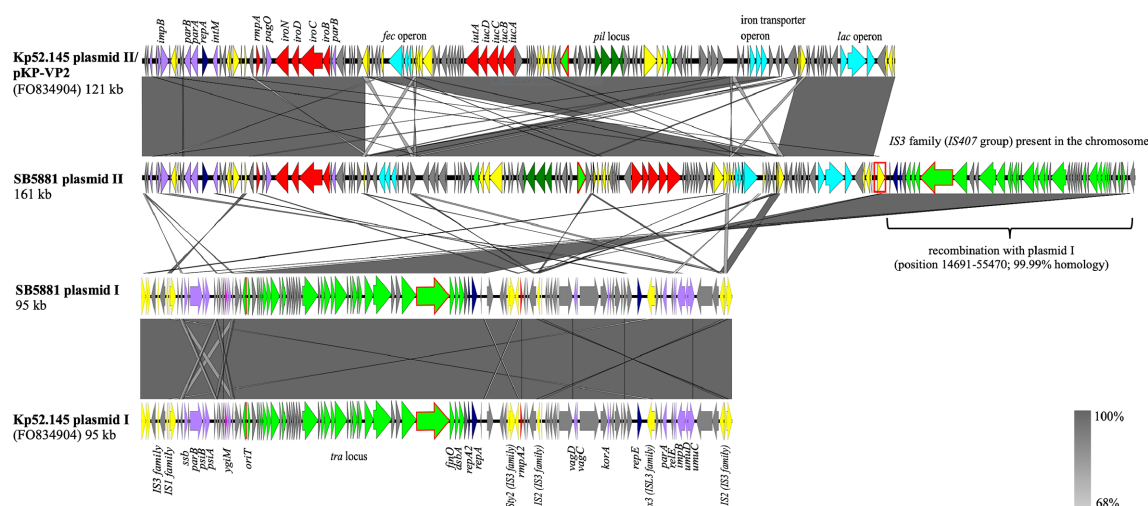
Fig. 1. Linear comparison of plasmid I and II from strain Kp52.145 and the ones from SB5881. The grey shading denotes shared regions of homology. ORFs are portrayed by arrows and coloured based on the predicted gene function: blue, replication; green, DNA transfer (associated with the tra locus – T4SS and T4CP systems); orange, origin of transfer site ( oriT ); light purple, partition, stability, and maintenance; yellow, mobile genetic elements; dark green, type IV pilus biosynthesis locus; red, virulence genes; cyan, iron transporter, lactose and fec operons; fuchsia, prophage-linked; light grey, other functions. Predicted relaxase is outlined in red. IS3 family (IS407 group) in the recombination region of plasmid I and II, originated from the chromosome of SB5881, is represented by a red box.
